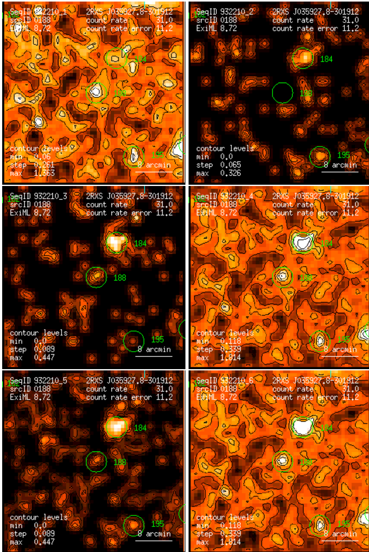
Figure 188: RASS 932210: detection 0188: band rate images, Gaussian filter: (1) PSPC channels 11 – 41, (2) 52 – 90, (3) 91 – 201, (4) 11 – 235, (5) 52 – 201, (6) 11 – 201. Broad band rates in counts/ks. Band rate contour levels in counts/ks/arcmin 2 .
