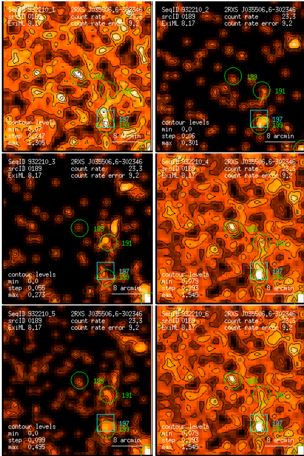
Figure 189: RASS 932210: detection 0189: band rate images, Gaussian filter: (1) PSPC channels 11 – 41, (2) 52 – 90, (3) 91 – 201, (4) 11 – 235, (5) 52 – 201, (6) 11 – 201. Broad band rates in counts/ks. Band rate contour levels in counts/ks/arcmin 2 .
