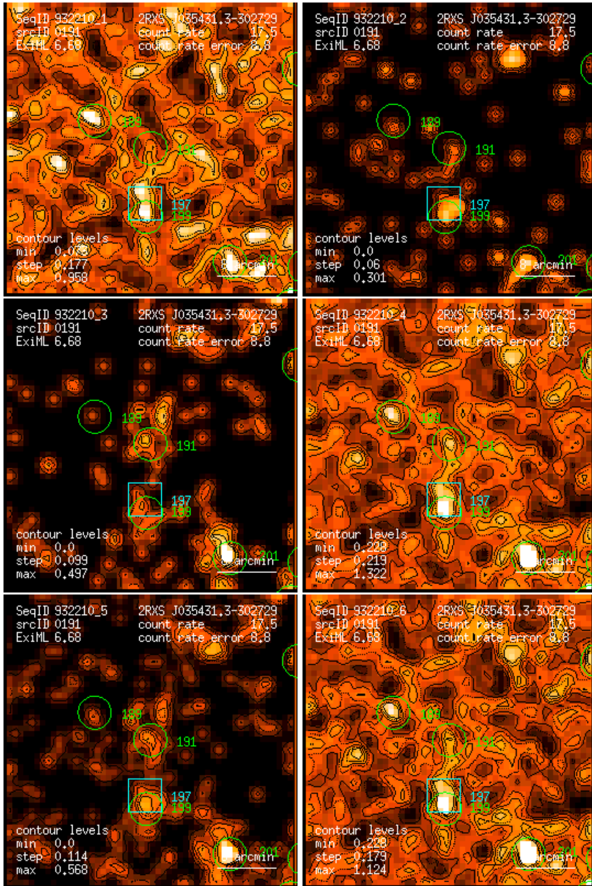
Figure 191: RASS 932210: detection 0191: band rate images, Gaussian filter: (1) PSPC channels 11 – 41, (2) 52 – 90, (3) 91 – 201, (4) 11 – 235, (5) 52 – 201, (6) 11 – 201. Broad band rates in counts/ks. Band rate contour levels in counts/ks/arcmin 2 .
