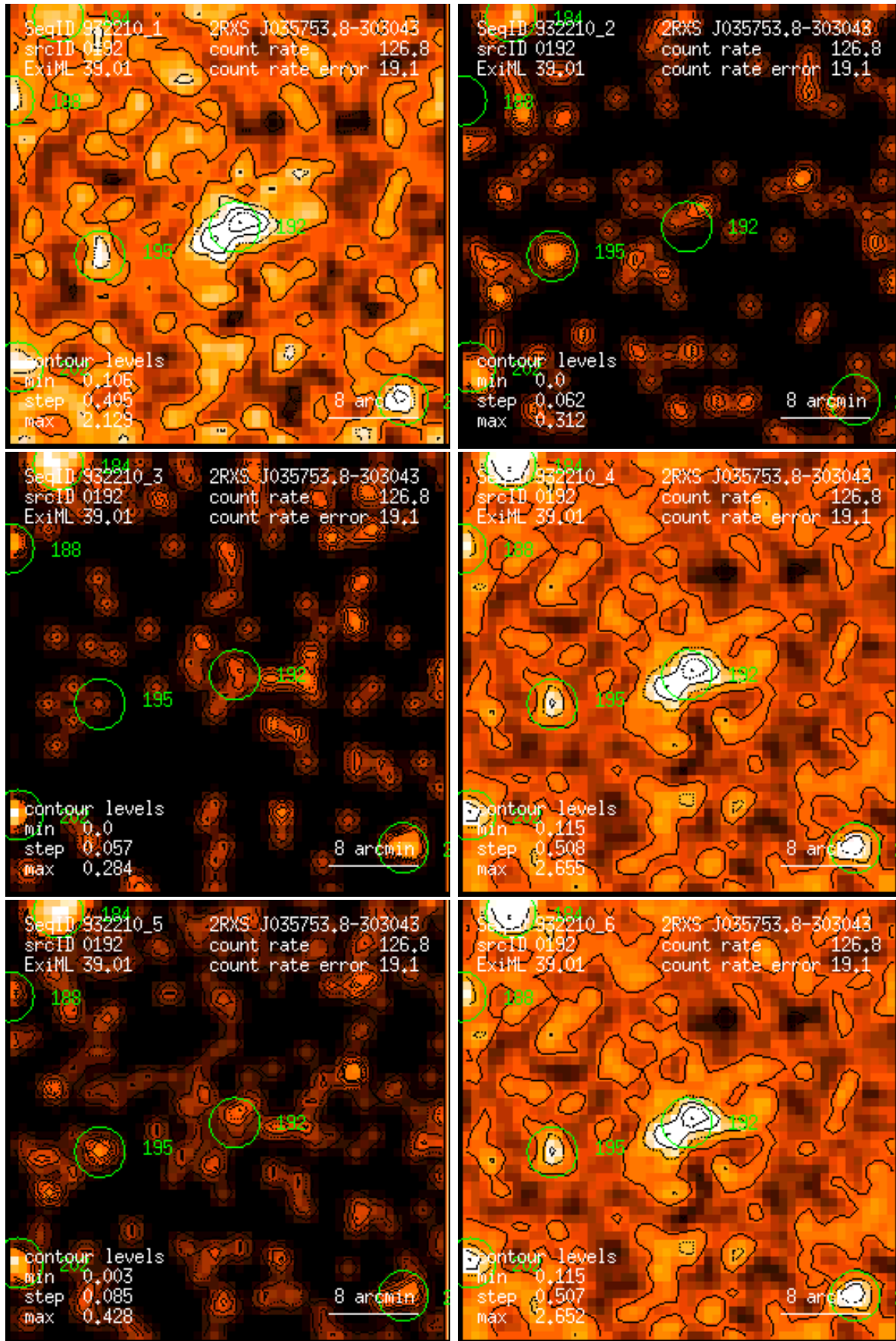
Figure 192: RASS 932210: detection 0192: band rate images, Gaussian filter: (1) PSPC channels 11 – 41, (2) 52 – 90, (3) 91 – 201, (4) 11 – 235, (5) 52 – 201, (6) 11 – 201. Broad band rates in counts/ks. Band rate contour levels in counts/ks/arcmin 2 .
