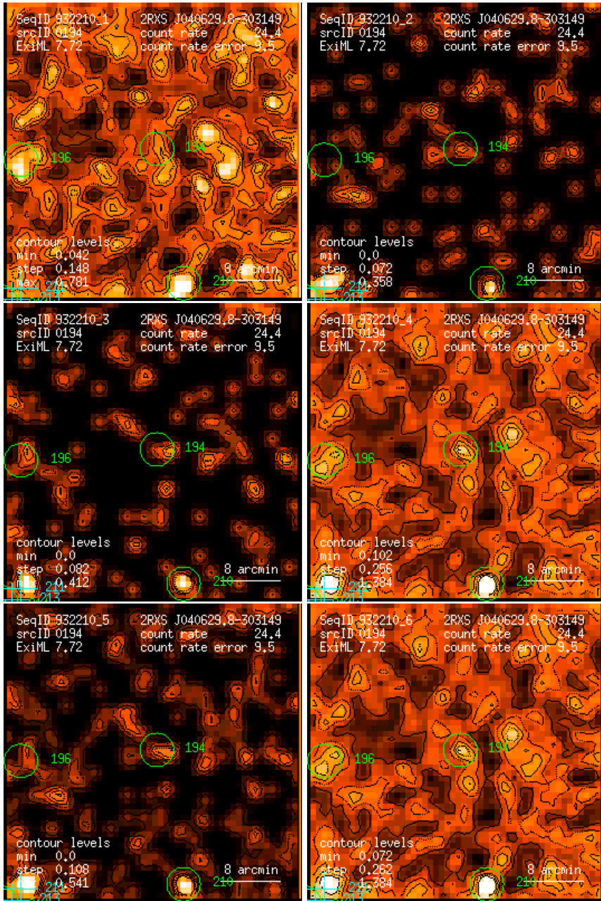
Figure 194: RASS 932210: detection 0194: band rate images, Gaussian filter: (1) PSPC channels 11 – 41, (2) 52 – 90, (3) 91 – 201, (4) 11 – 235, (5) 52 – 201, (6) 11 – 201. Broad band rates in counts/ks. Band rate contour levels in counts/ks/arcmin 2 .
