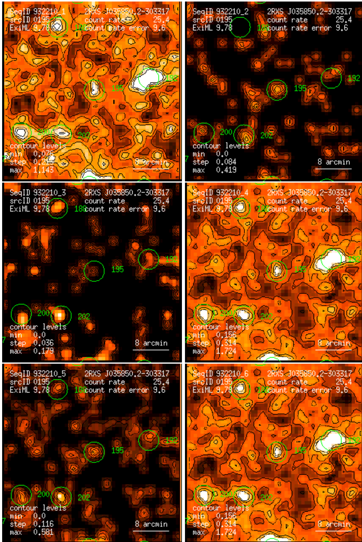
Figure 195: RASS 932210: detection 0195: band rate images, Gaussian filter: (1) PSPC channels 11 – 41, (2) 52 – 90, (3) 91 – 201, (4) 11 – 235, (5) 52 – 201, (6) 11 – 201. Broad band rates in counts/ks. Band rate contour levels in counts/ks/arcmin 2 .
