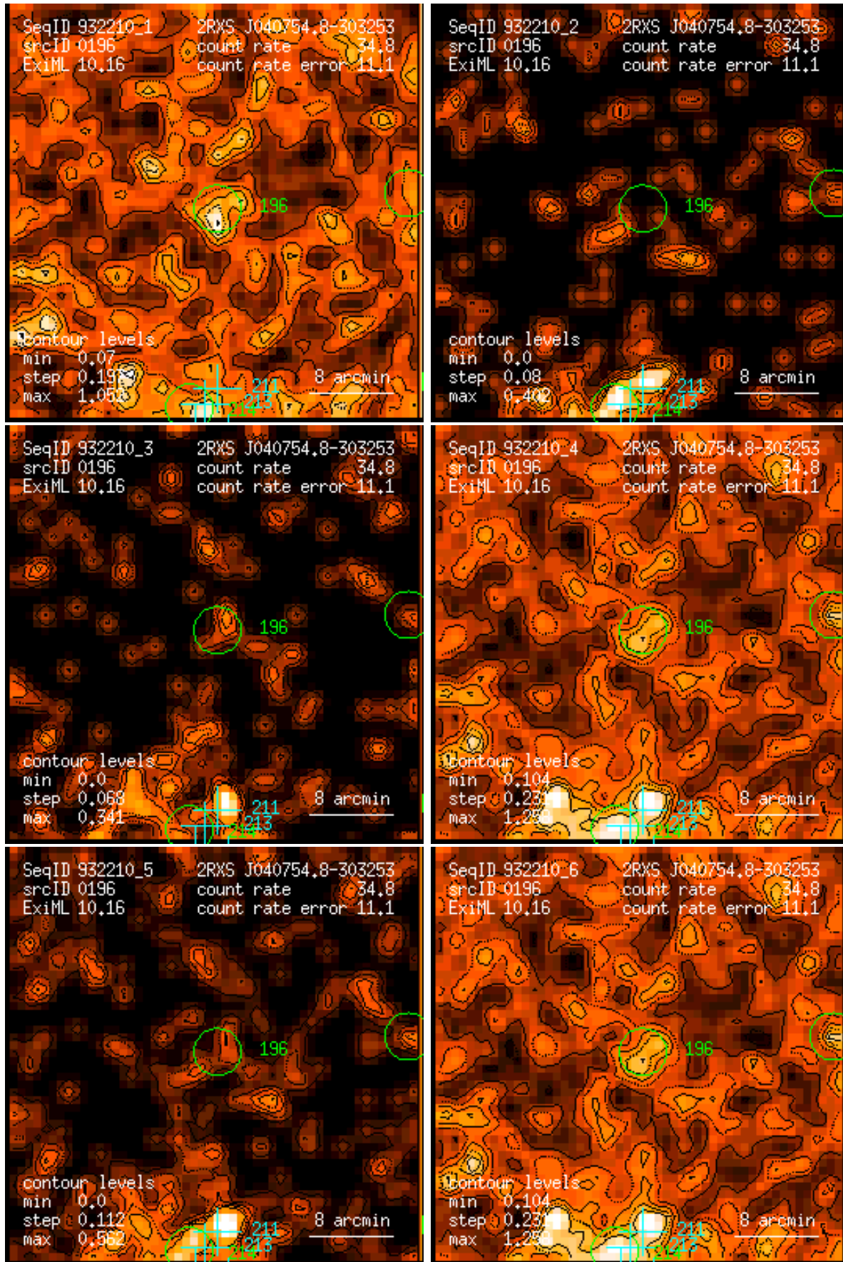
Figure 196: RASS 932210: detection 0196: band rate images, Gaussian filter: (1) PSPC channels 11 – 41, (2) 52 – 90, (3) 91 – 201, (4) 11 – 235, (5) 52 – 201, (6) 11 – 201. Broad band rates in counts/ks. Band rate contour levels in counts/ks/arcmin 2 .
