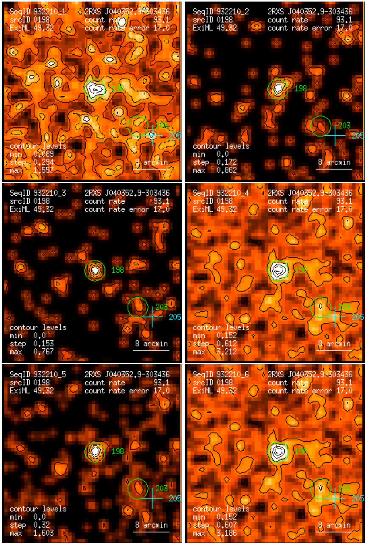
Figure 198: RASS 932210: detection 0198: band rate images, Gaussian filter: (1) PSPC channels 11 – 41, (2) 52 – 90, (3) 91 – 201, (4) 11 – 235, (5) 52 – 201, (6) 11 – 201. Broad band rates in counts/ks. Band rate contour levels in counts/ks/arcmin 2 .
