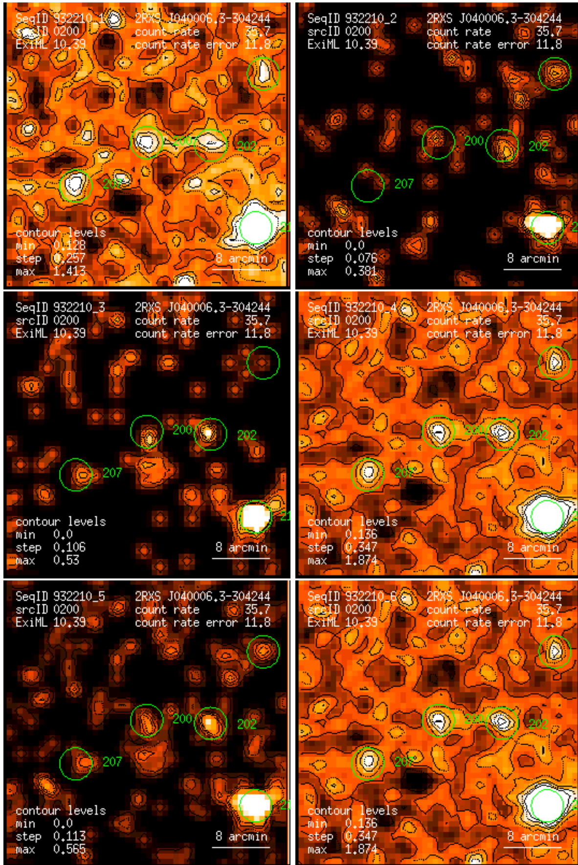
Figure 200: RASS 932210: detection 0200: band rate images, Gaussian filter: (1) PSPC channels 11 – 41, (2) 52 – 90, (3) 91 – 201, (4) 11 – 235, (5) 52 – 201, (6) 11 – 201. Broad band rates in counts/ks. Band rate contour levels in counts/ks/arcmin 2 .
