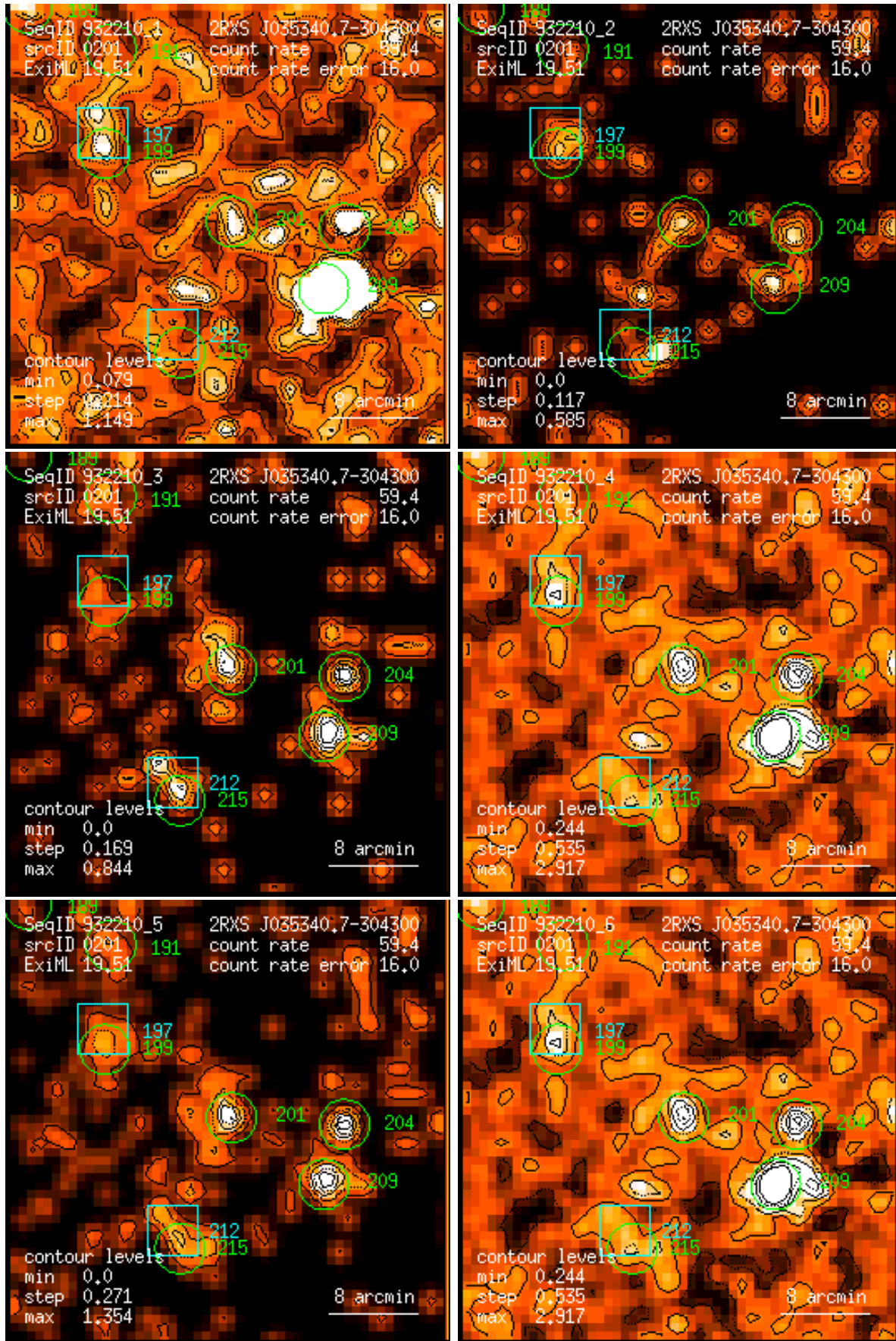
Figure 201: RASS 932210: detection 0201: band rate images, Gaussian filter: (1) PSPC channels 11 – 41, (2) 52 – 90, (3) 91 – 201, (4) 11 – 235, (5) 52 – 201, (6) 11 – 201. Broad band rates in counts/ks. Band rate contour levels in counts/ks/arcmin 2 .
