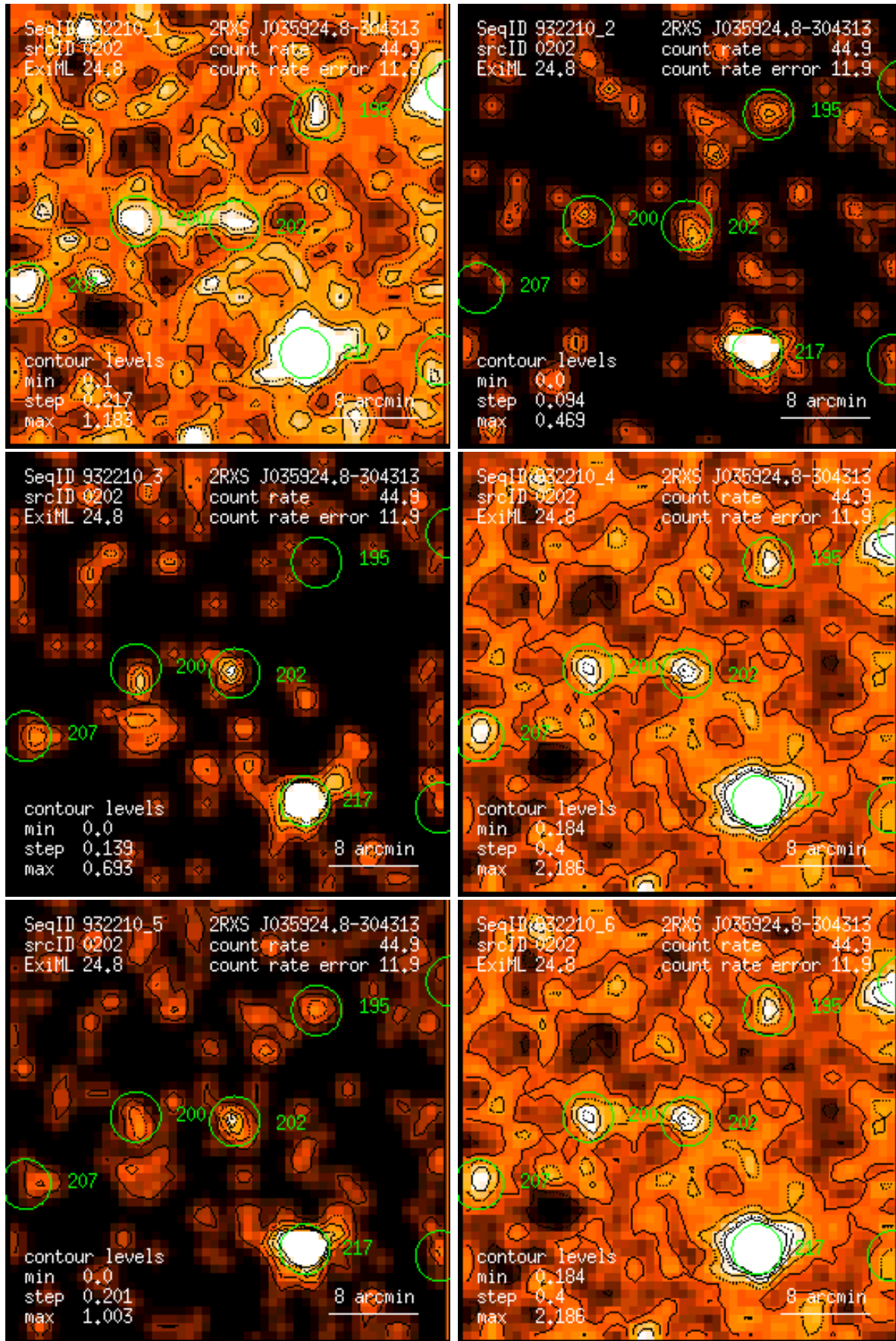
Figure 202: RASS 932210: detection 0202: band rate images, Gaussian filter: (1) PSPC channels 11 – 41, (2) 52 – 90, (3) 91 – 201, (4) 11 – 235, (5) 52 – 201, (6) 11 – 201. Broad band rates in counts/ks. Band rate contour levels in counts/ks/arcmin 2 .
