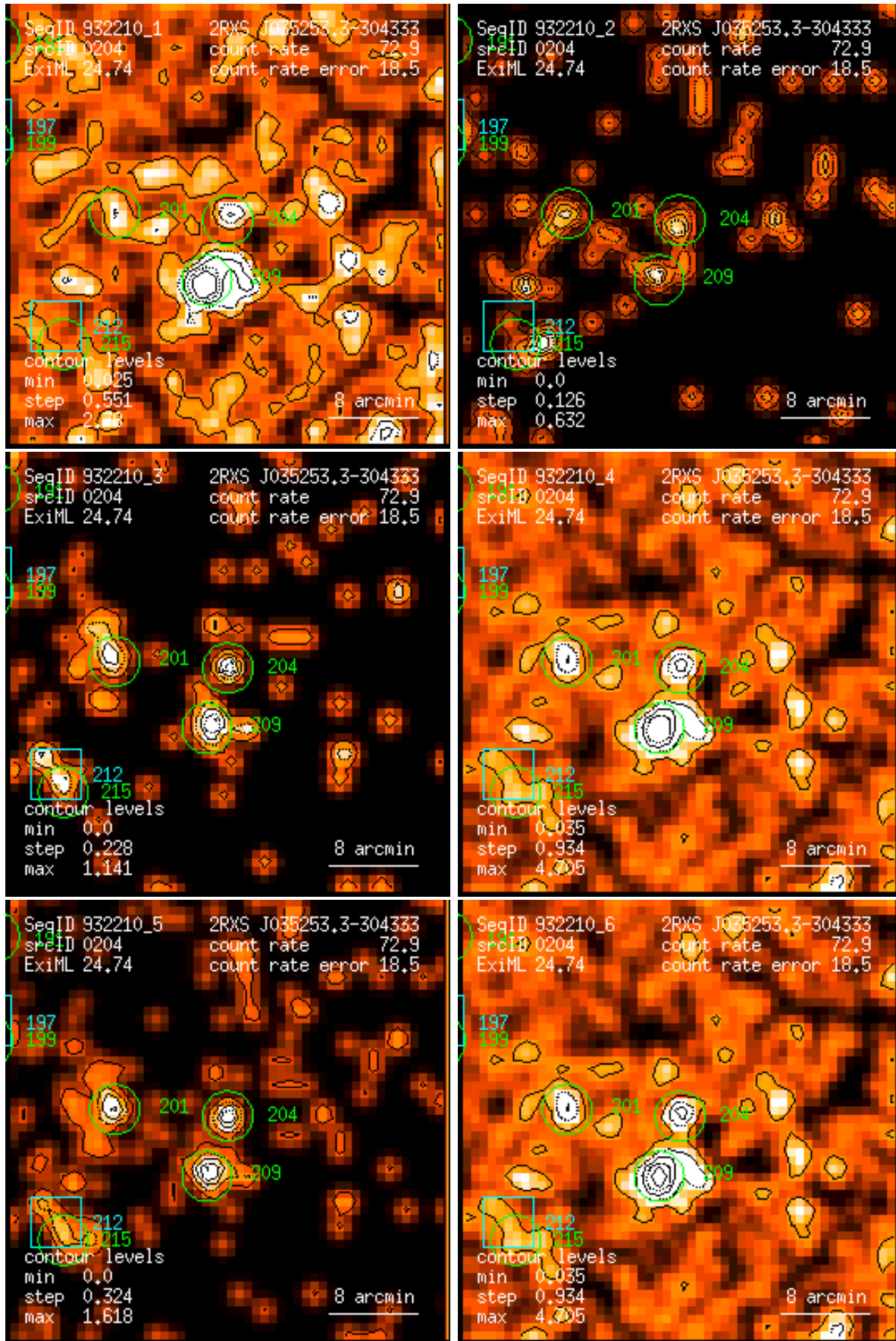
Figure 204: RASS 932210: detection 0204: band rate images, Gaussian filter: (1) PSPC channels 11 – 41, (2) 52 – 90, (3) 91 – 201, (4) 11 – 235, (5) 52 – 201, (6) 11 – 201. Broad band rates in counts/ks. Band rate contour levels in counts/ks/arcmin 2 .
