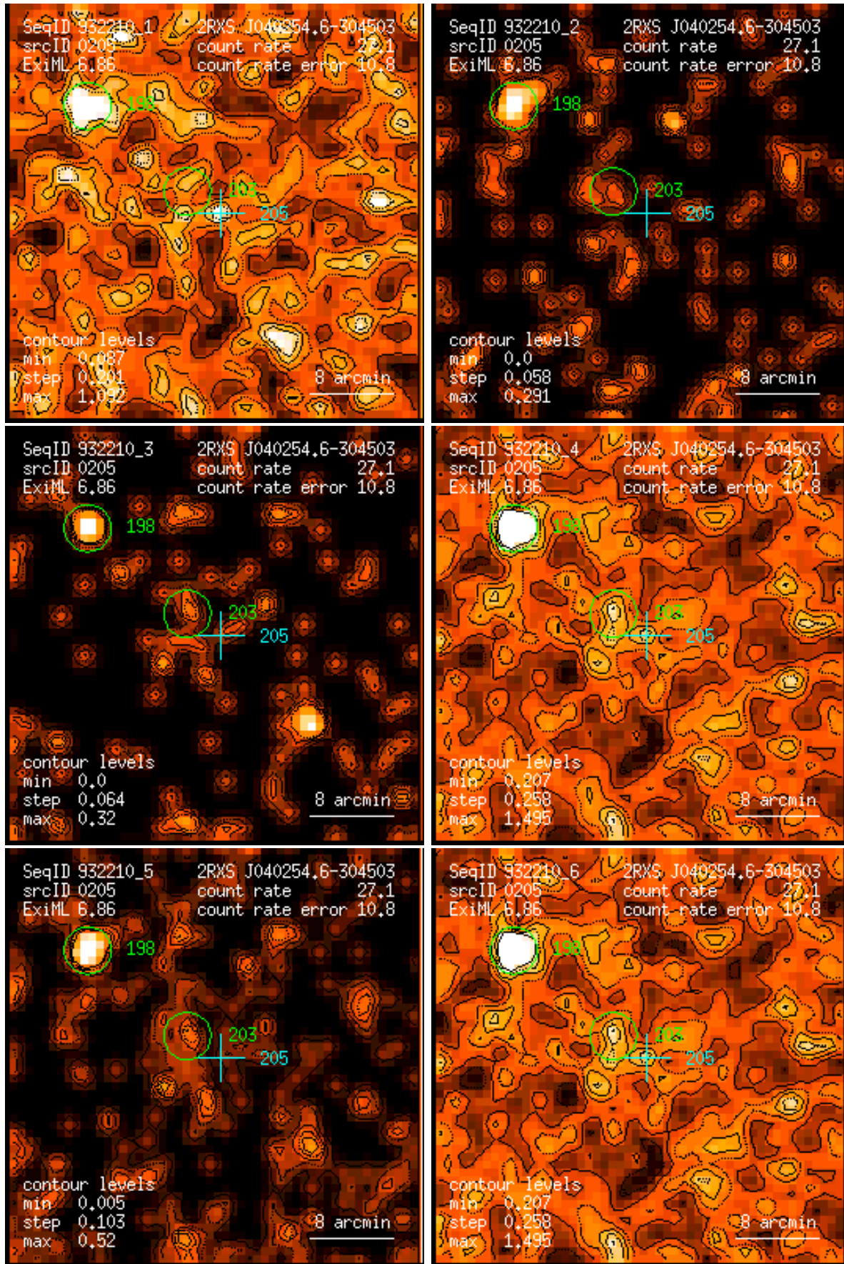
Figure 205: RASS 932210: detection 0205: band rate images, Gaussian filter: (1) PSPC channels 11 – 41, (2) 52 – 90, (3) 91 – 201, (4) 11 – 235, (5) 52 – 201, (6) 11 – 201. Broad band rates in counts/ks. Band rate contour levels in counts/ks/arcmin 2 .
