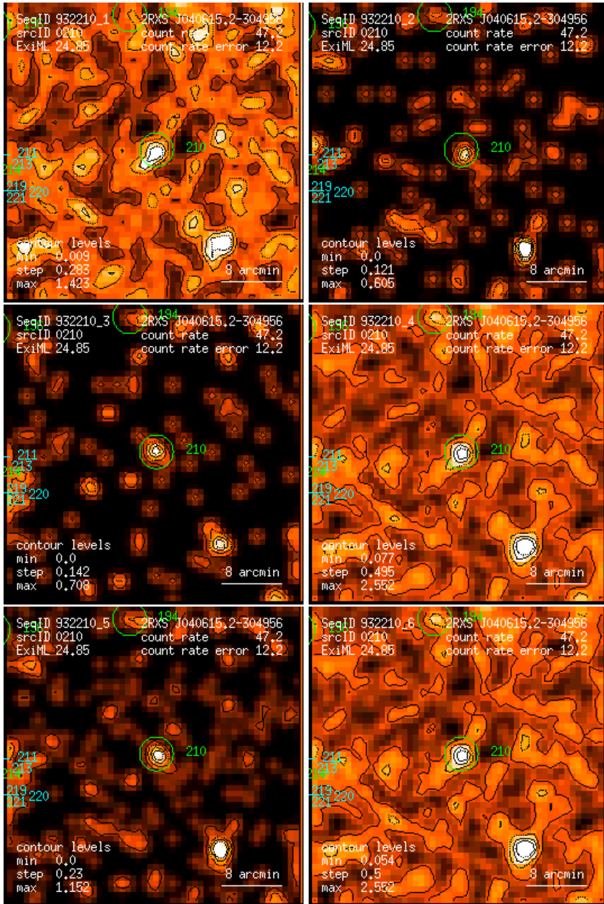
Figure 210: RASS 932210: detection 0210: band rate images, Gaussian filter: (1) PSPC channels 11 – 41, (2) 52 – 90, (3) 91 – 201, (4) 11 – 235, (5) 52 – 201, (6) 11 – 201. Broad band rates in counts/ks. Band rate contour levels in counts/ks/arcmin 2 .
