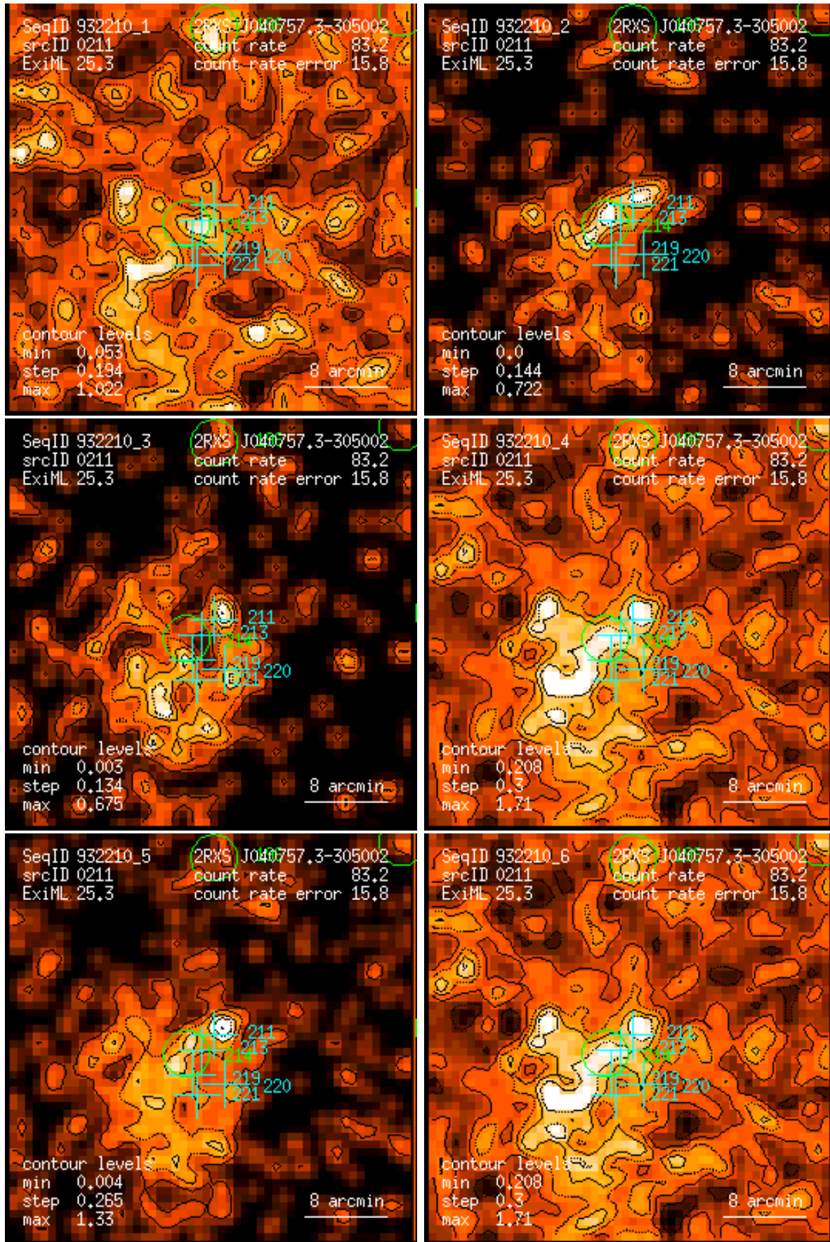
Figure 211: RASS 932210: detection 0211: band rate images, Gaussian filter: (1) PSPC channels 11 – 41, (2) 52 – 90, (3) 91 – 201, (4) 11 – 235, (5) 52 – 201, (6) 11 – 201. Broad band rates in counts/ks. Band rate contour levels in counts/ks/arcmin 2 .
