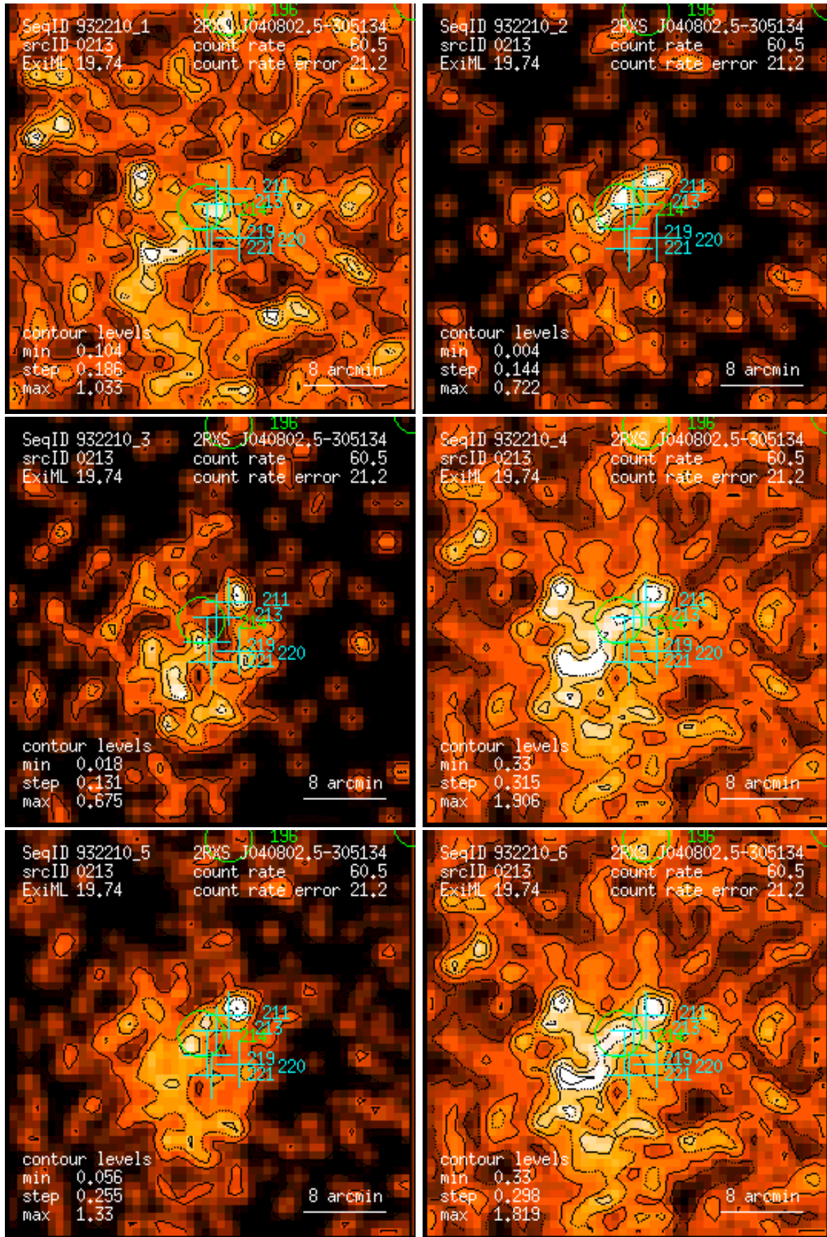
Figure 213: RASS 932210: detection 0213: band rate images, Gaussian filter: (1) PSPC channels 11 – 41, (2) 52 – 90, (3) 91 – 201, (4) 11 – 235, (5) 52 – 201, (6) 11 – 201. Broad band rates in counts/ks. Band rate contour levels in counts/ks/arcmin 2 .
