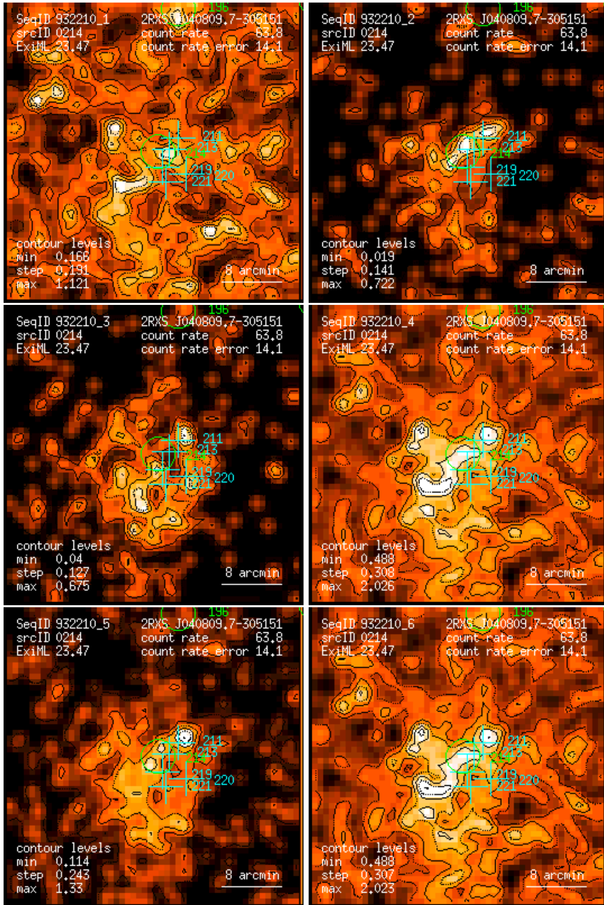
Figure 214: RASS 932210: detection 0214: band rate images, Gaussian filter: (1) PSPC channels 11 – 41, (2) 52 – 90, (3) 91 – 201, (4) 11 – 235, (5) 52 – 201, (6) 11 – 201. Broad band rates in counts/ks. Band rate contour levels in counts/ks/arcmin 2 .
