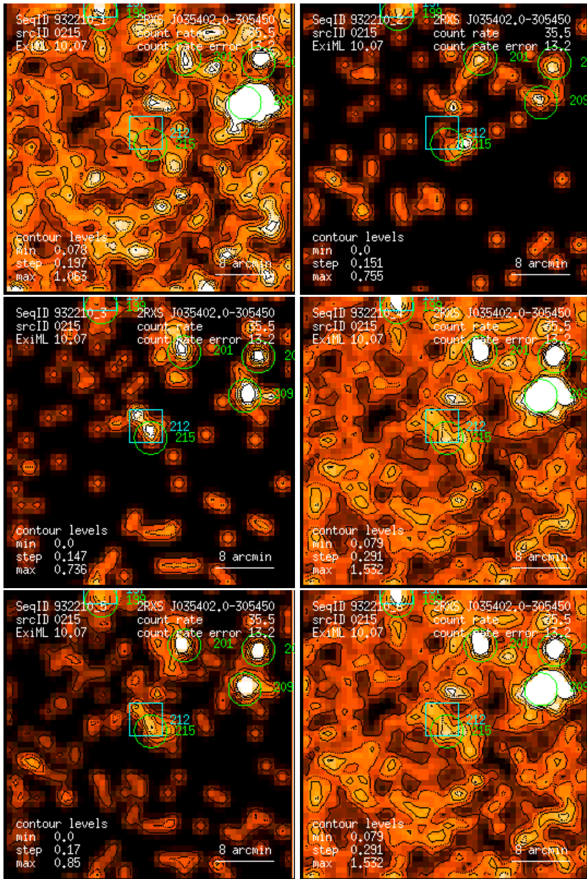
Figure 215: RASS 932210: detection 0215: band rate images, Gaussian filter: (1) PSPC channels 11 – 41, (2) 52 – 90, (3) 91 – 201, (4) 11 – 235, (5) 52 – 201, (6) 11 – 201. Broad band rates in counts/ks. Band rate contour levels in counts/ks/arcmin 2 .
