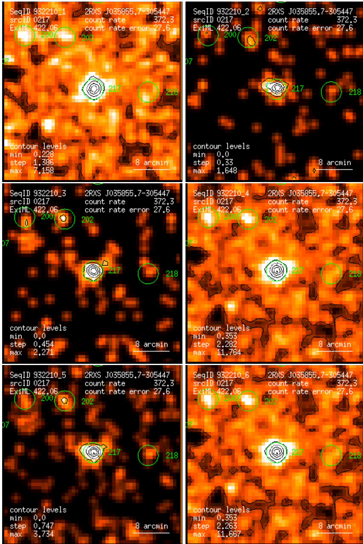
Figure 217: RASS 932210: detection 0217: band rate images, Gaussian filter: (1) PSPC channels 11 – 41, (2) 52 – 90, (3) 91 – 201, (4) 11 – 235, (5) 52 – 201, (6) 11 – 201. Broad band rates in counts/ks. Band rate contour levels in counts/ks/arcmin 2 .
