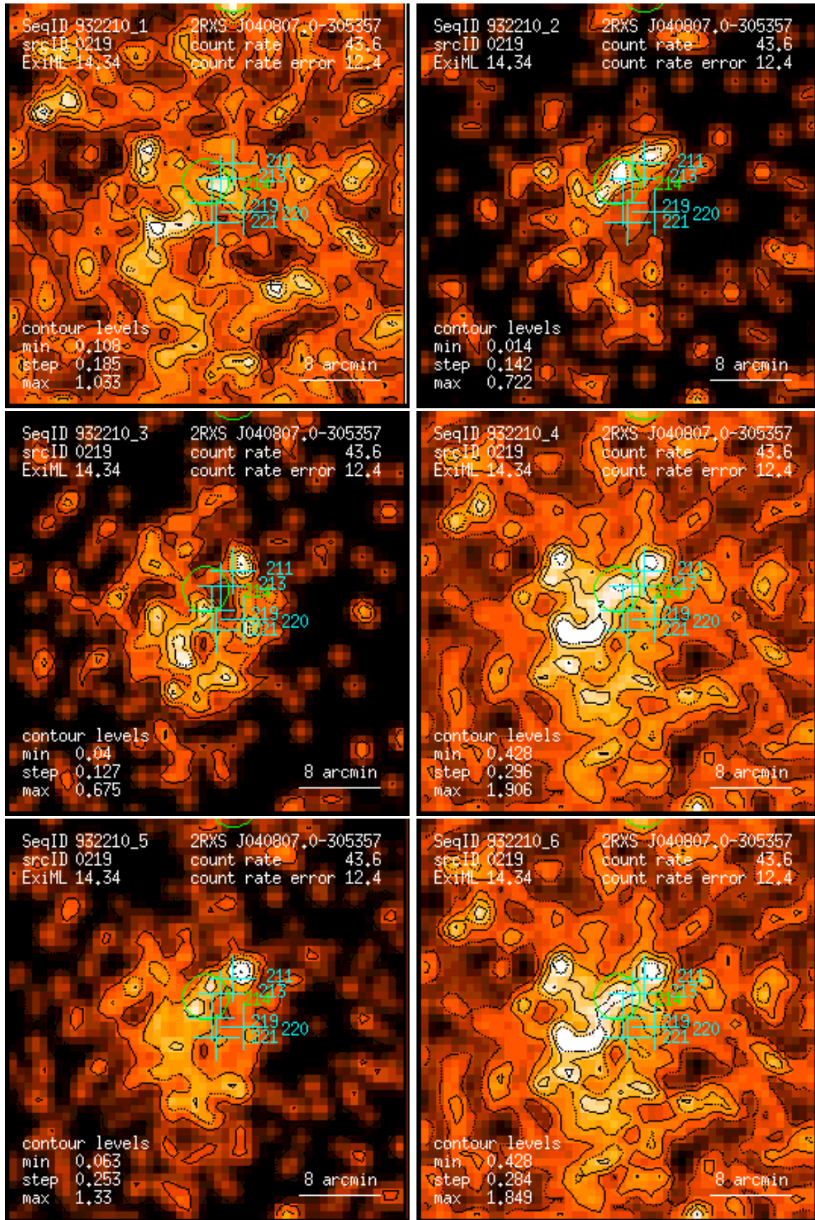
Figure 219: RASS 932210: detection 0219: band rate images, Gaussian filter: (1) PSPC channels 11 – 41, (2) 52 – 90, (3) 91 – 201, (4) 11 – 235, (5) 52 – 201, (6) 11 – 201. Broad band rates in counts/ks. Band rate contour levels in counts/ks/arcmin 2 .
