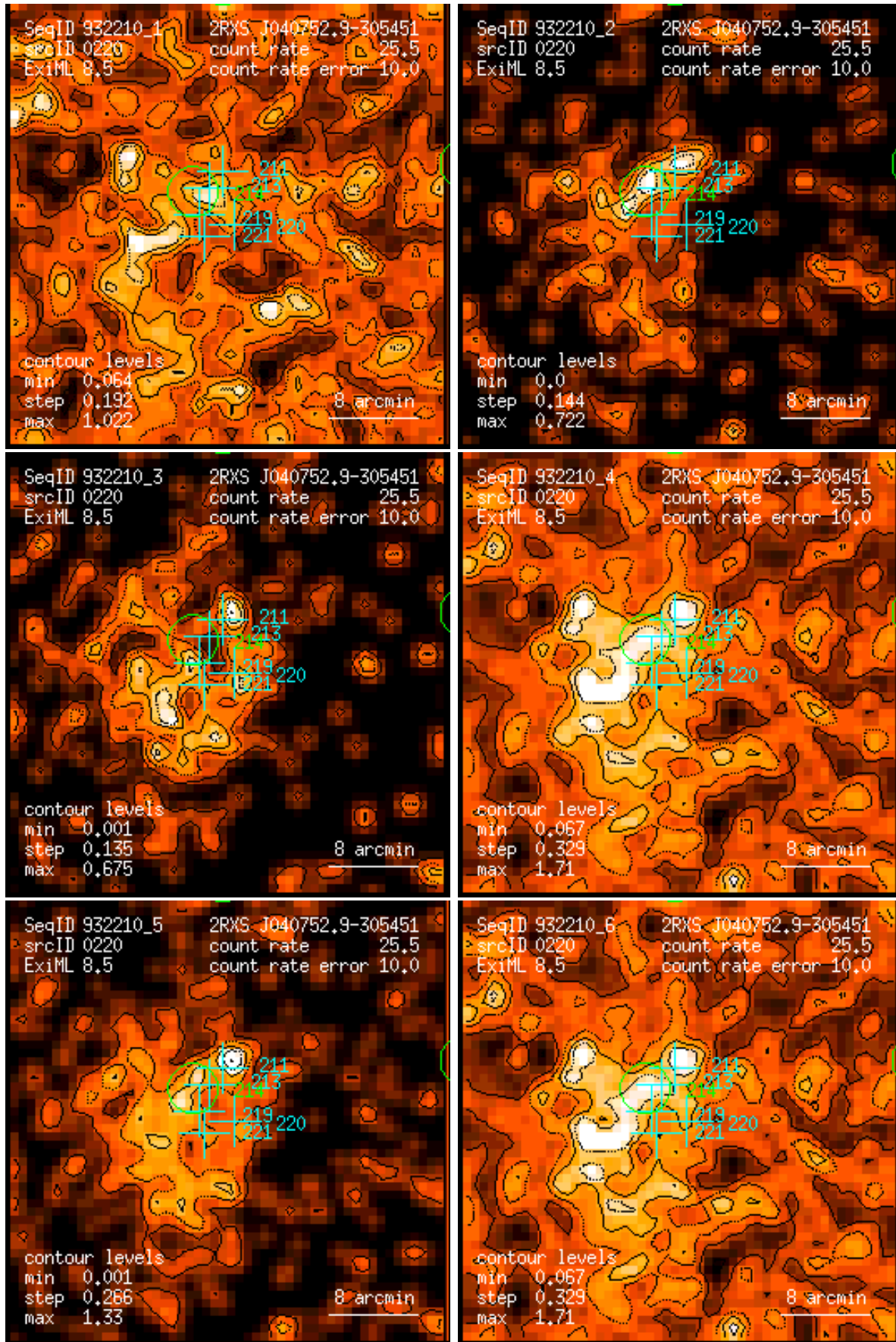
Figure 220: RASS 932210: detection 0220: band rate images, Gaussian filter: (1) PSPC channels 11 – 41, (2) 52 – 90, (3) 91 – 201, (4) 11 – 235, (5) 52 – 201, (6) 11 – 201. Broad band rates in counts/ks. Band rate contour levels in counts/ks/arcmin 2 .
