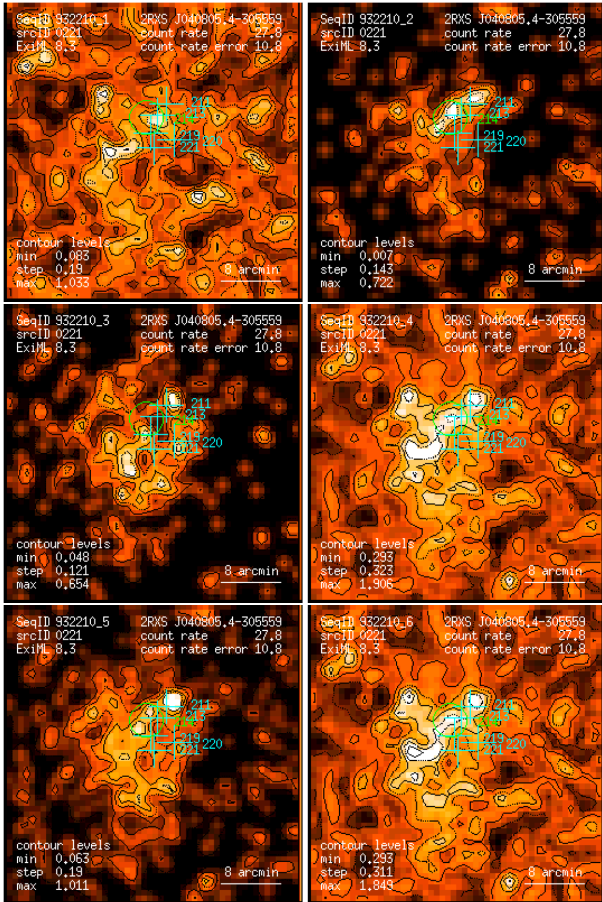
Figure 221: RASS 932210: detection 0221: band rate images, Gaussian filter: (1) PSPC channels 11 – 41, (2) 52 – 90, (3) 91 – 201, (4) 11 – 235, (5) 52 – 201, (6) 11 – 201. Broad band rates in counts/ks. Band rate contour levels in counts/ks/arcmin 2 .
