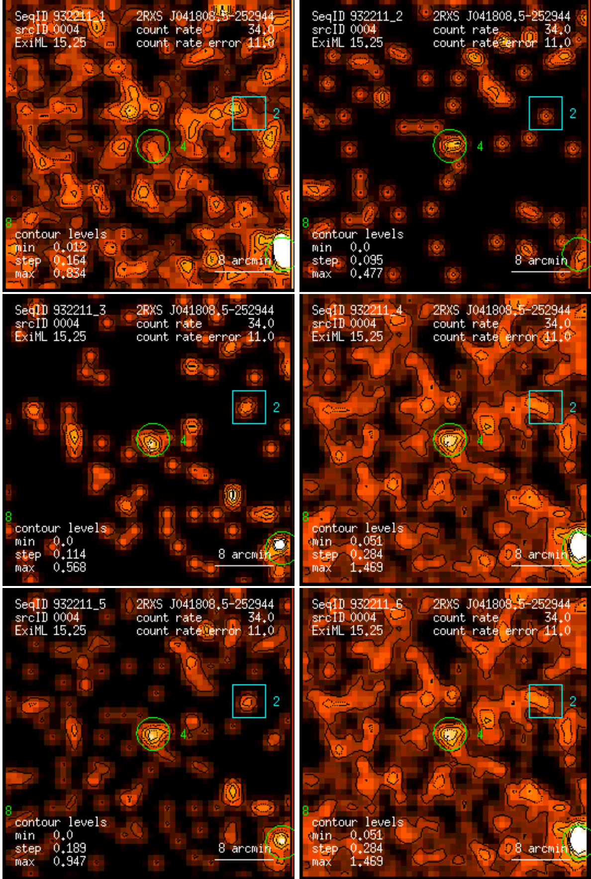
Figure 4: RASS 932211: detection 0004: band rate images, Gaussian filter: (1) PSPC channels 11 – 41, (2) 52 – 90, (3) 91 – 201, (4) 11 – 235, (5) 52 – 201, (6) 11 – 201. Broad band rates in counts/ks. Band rate contour levels in counts/ks/arcmin 2 .
