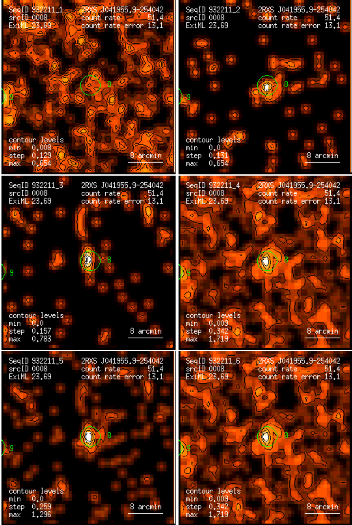
Figure 8: RASS 932211: detection 0008: band rate images, Gaussian filter: (1) PSPC channels 11 – 41, (2) 52 – 90, (3) 91 – 201, (4) 11 – 235, (5) 52 – 201, (6) 11 – 201. Broad band rates in counts/ks. Band rate contour levels in counts/ks/arcmin 2 .
