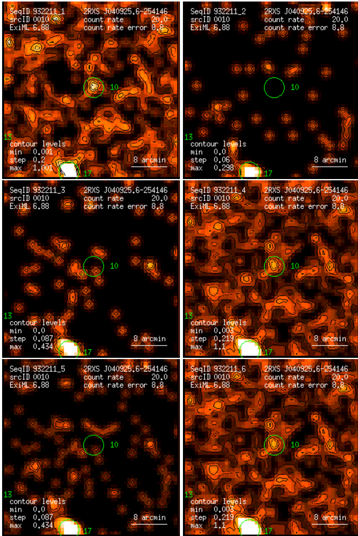
Figure 10: RASS 932211: detection 0010: band rate images, Gaussian filter: (1) PSPC channels 11 – 41, (2) 52 – 90, (3) 91 – 201, (4) 11 – 235, (5) 52 – 201, (6) 11 – 201. Broad band rates in counts/ks. Band rate contour levels in counts/ks/arcmin 2 .
