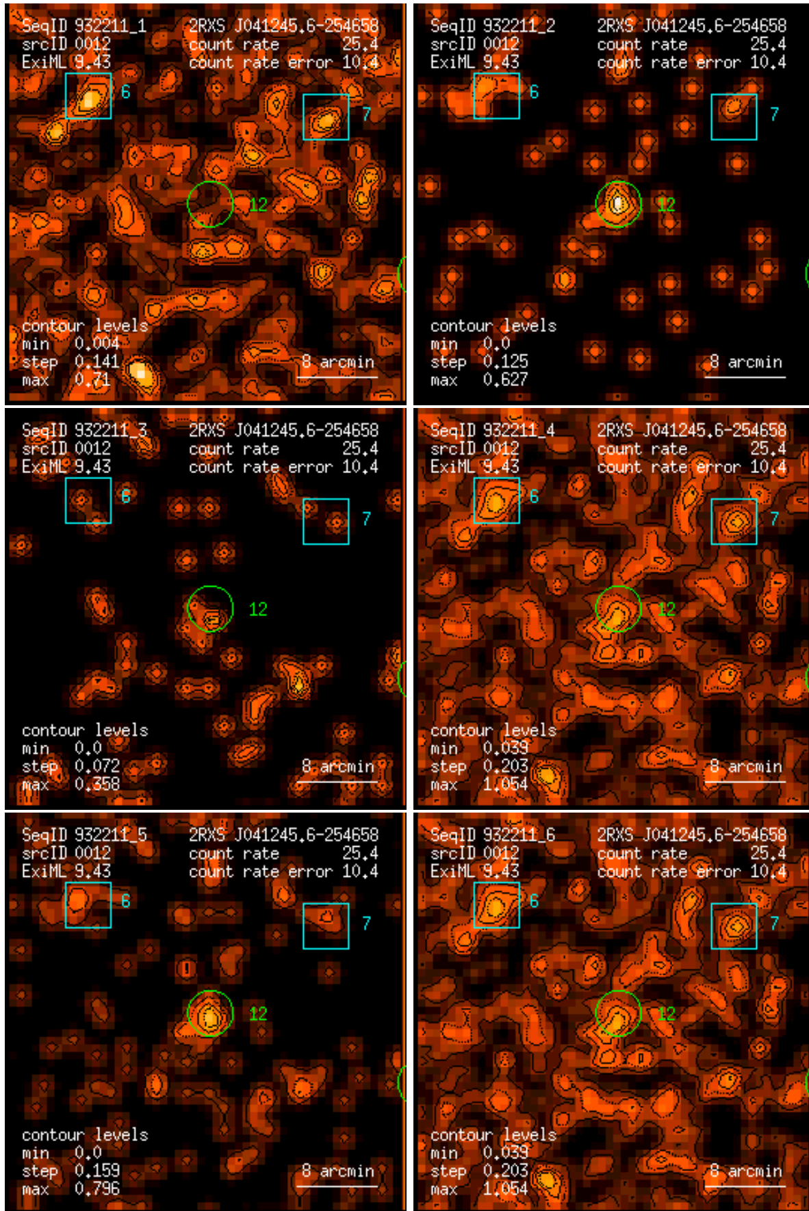
Figure 12: RASS 932211: detection 0012: band rate images, Gaussian filter: (1) PSPC channels 11 – 41, (2) 52 – 90, (3) 91 – 201, (4) 11 – 235, (5) 52 – 201, (6) 11 – 201. Broad band rates in counts/ks. Band rate contour levels in counts/ks/arcmin 2 .
