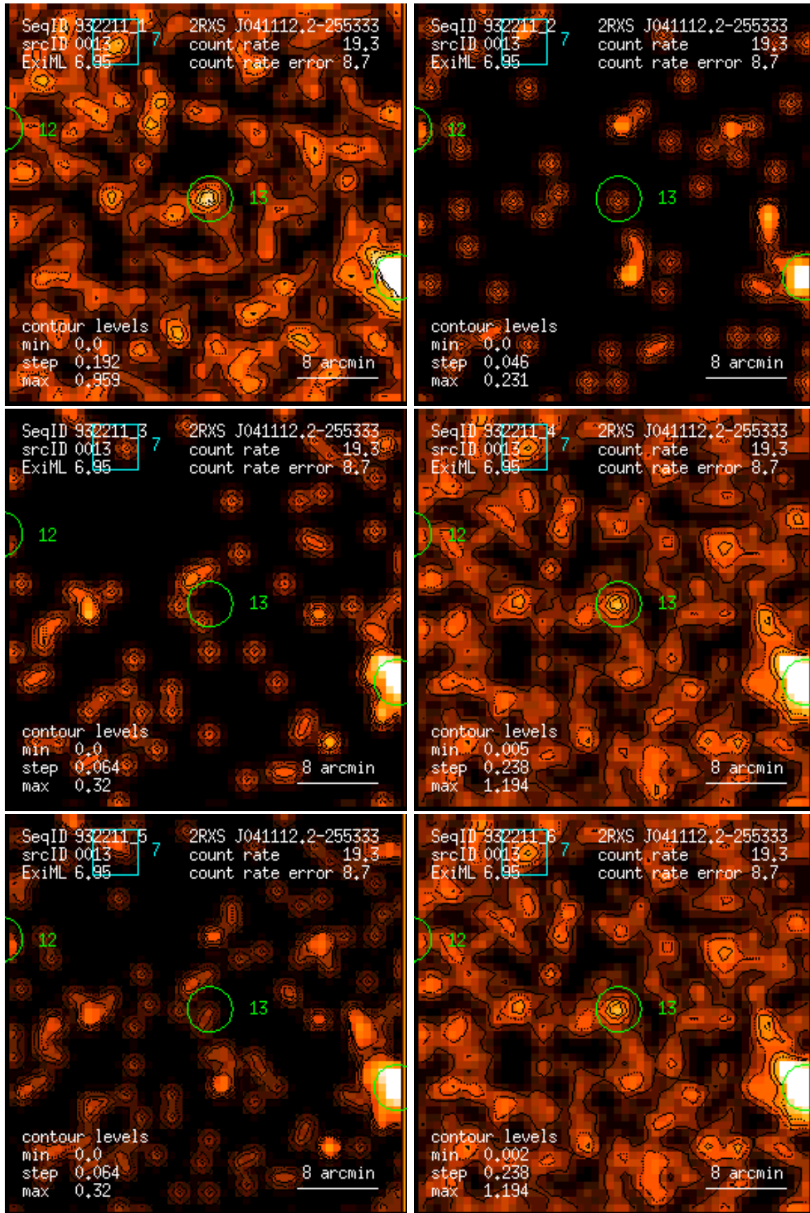
Figure 13: RASS 932211: detection 0013: band rate images, Gaussian filter: (1) PSPC channels 11 – 41, (2) 52 – 90, (3) 91 – 201, (4) 11 – 235, (5) 52 – 201, (6) 11 – 201. Broad band rates in counts/ks. Band rate contour levels in counts/ks/arcmin 2 .
