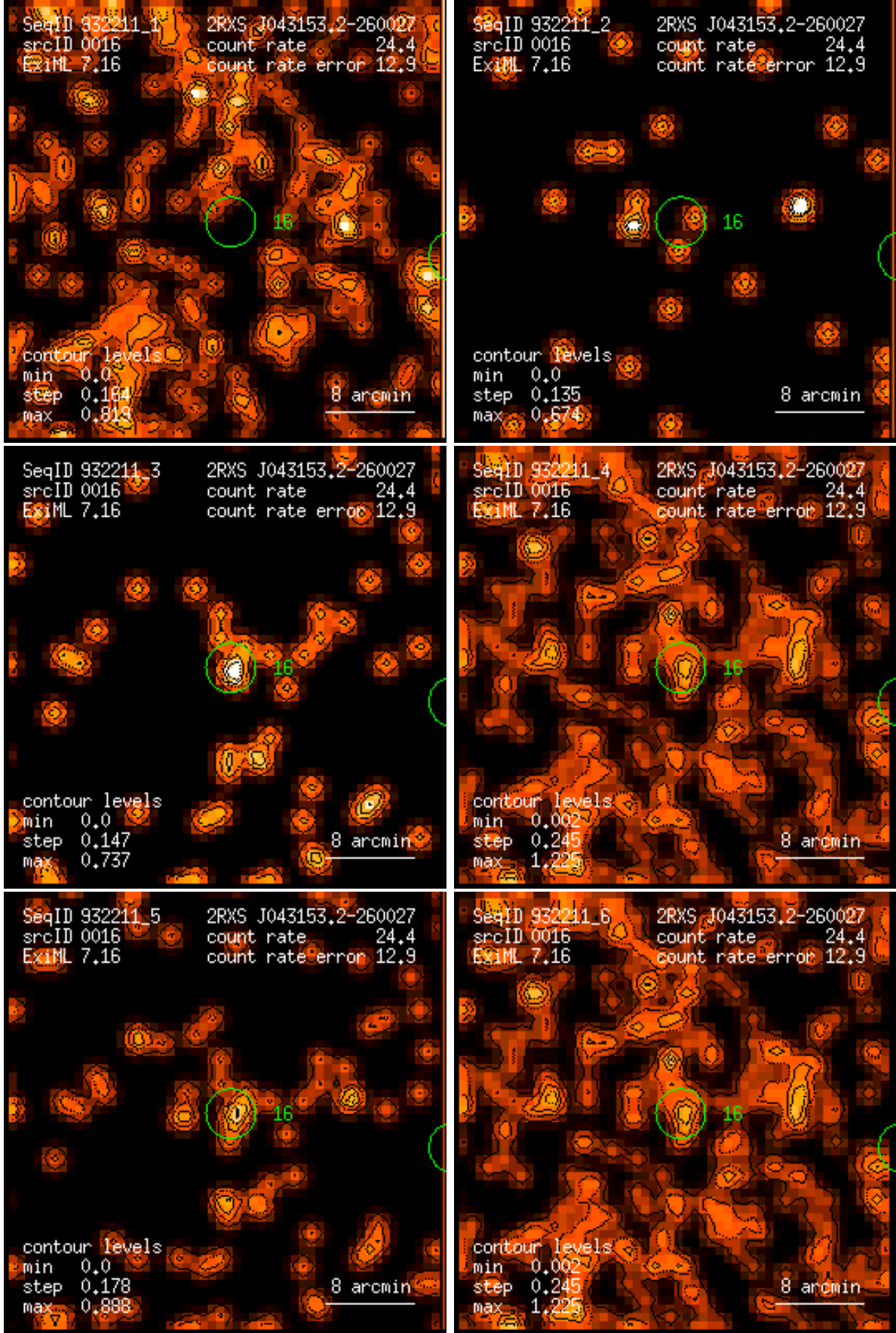
Figure 16: RASS 932211: detection 0016: band rate images, Gaussian filter: (1) PSPC channels 11 – 41, (2) 52 – 90, (3) 91 – 201, (4) 11 – 235, (5) 52 – 201, (6) 11 – 201. Broad band rates in counts/ks. Band rate contour levels in counts/ks/arcmin 2 .
