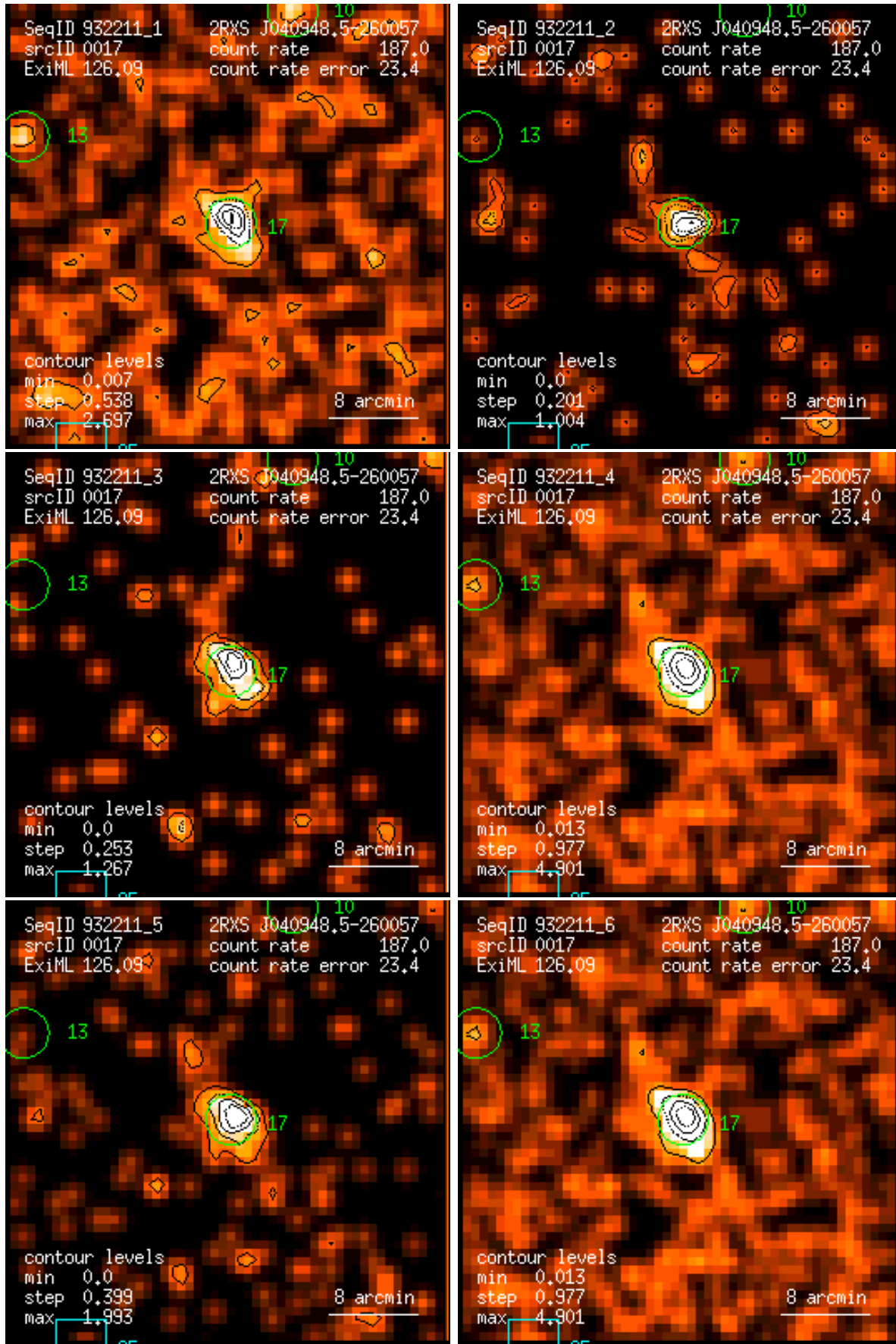
Figure 17: RASS 932211: detection 0017: band rate images, Gaussian filter: (1) PSPC channels 11 – 41, (2) 52 – 90, (3) 91 – 201, (4) 11 – 235, (5) 52 – 201, (6) 11 – 201. Broad band rates in counts/ks. Band rate contour levels in counts/ks/arcmin 2 .
