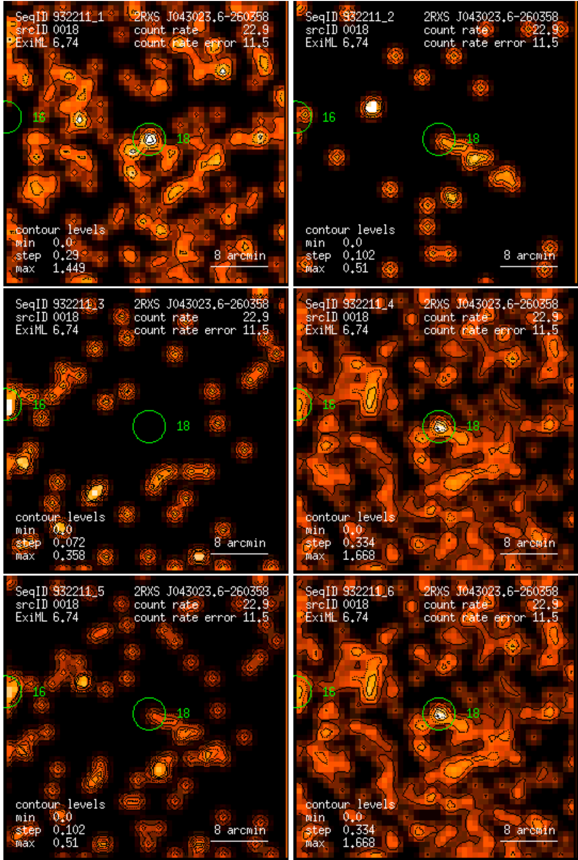
Figure 18: RASS 932211: detection 0018: band rate images, Gaussian filter: (1) PSPC channels 11 – 41, (2) 52 – 90, (3) 91 – 201, (4) 11 – 235, (5) 52 – 201, (6) 11 – 201. Broad band rates in counts/ks. Band rate contour levels in counts/ks/arcmin 2 .
