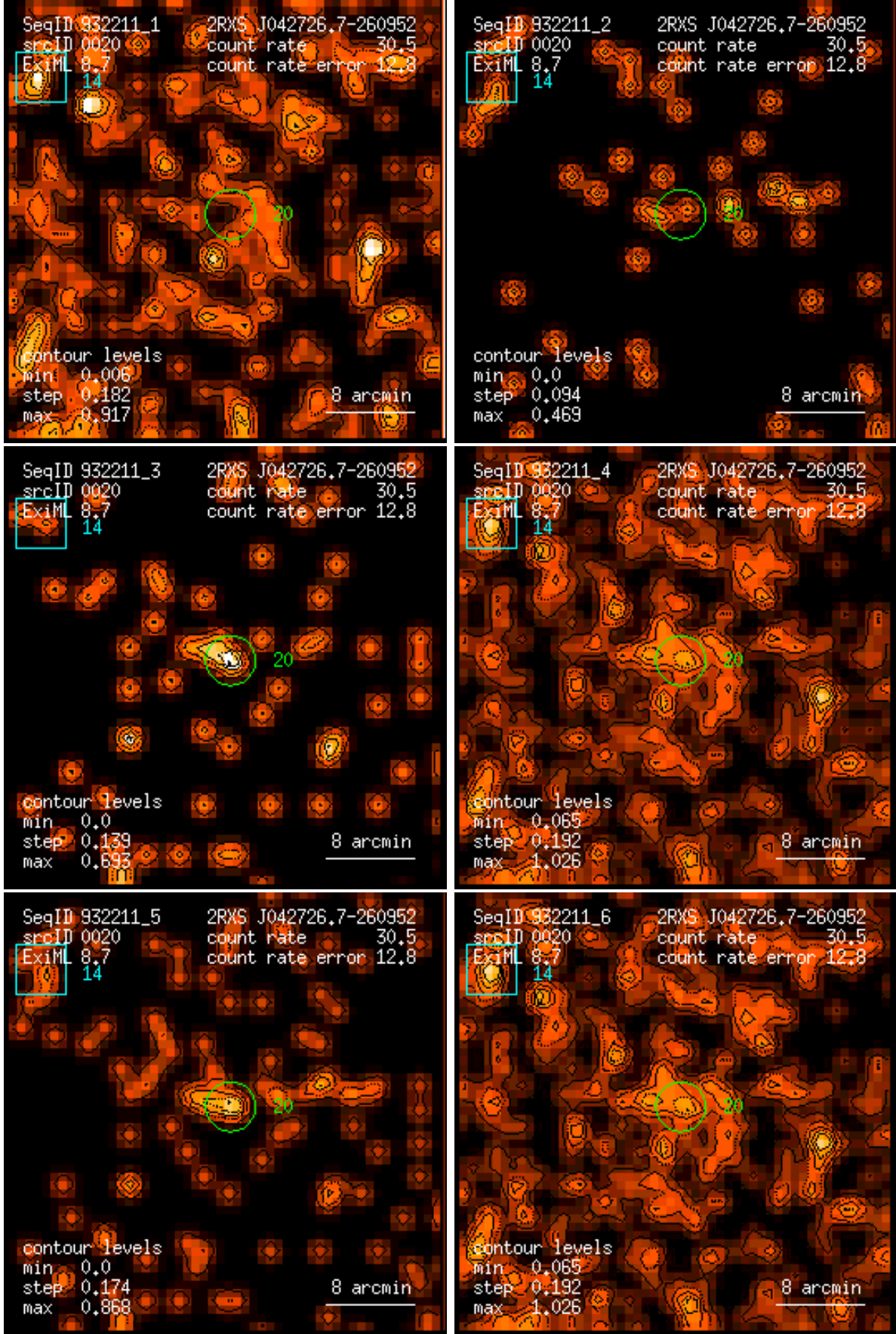
Figure 20: RASS 932211: detection 0020: band rate images, Gaussian filter: (1) PSPC channels 11 – 41, (2) 52 – 90, (3) 91 – 201, (4) 11 – 235, (5) 52 – 201, (6) 11 – 201. Broad band rates in counts/ks. Band rate contour levels in counts/ks/arcmin 2 .
