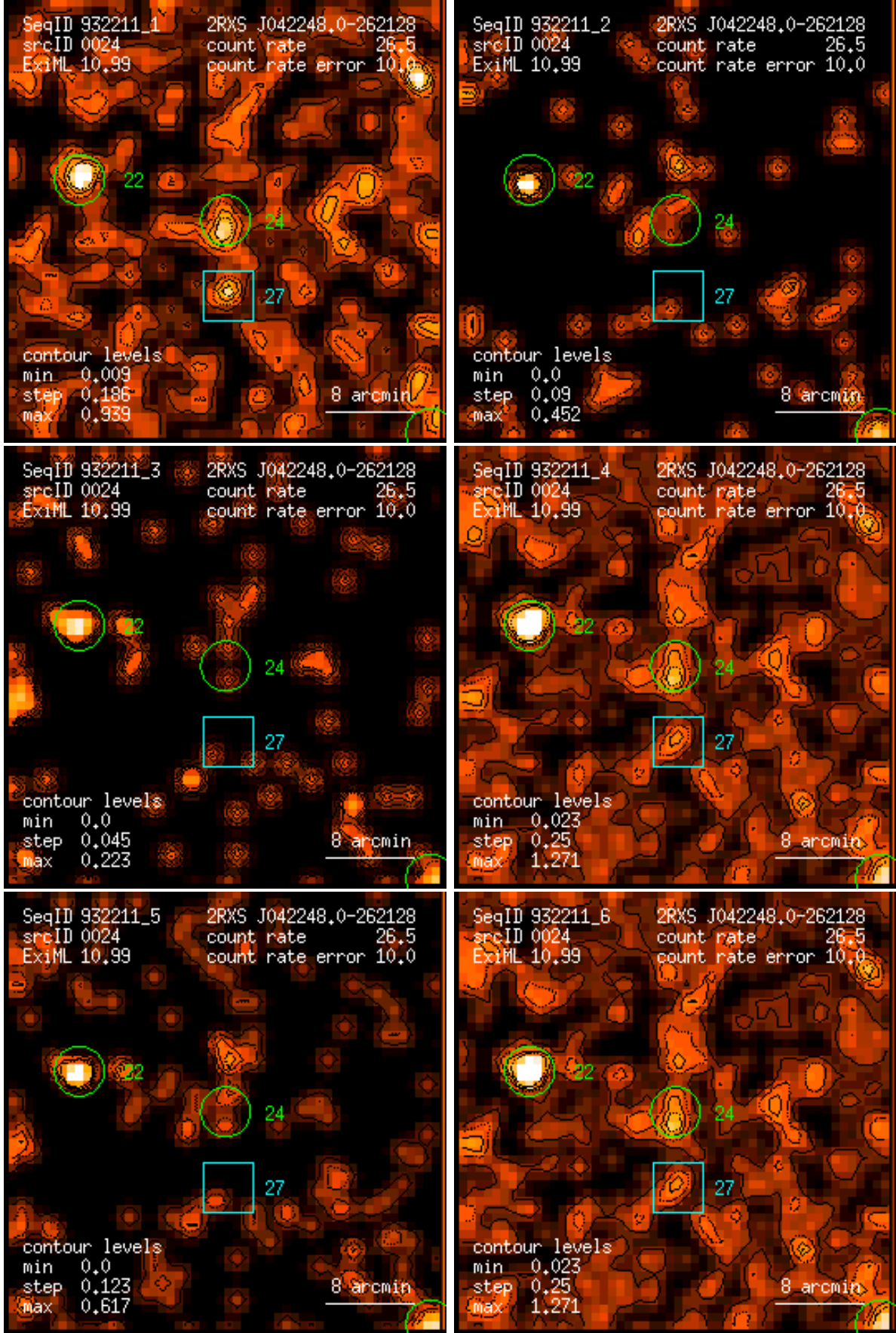
Figure 24: RASS 932211: detection 0024: band rate images, Gaussian filter: (1) PSPC channels 11 – 41, (2) 52 – 90, (3) 91 – 201, (4) 11 – 235, (5) 52 – 201, (6) 11 – 201. Broad band rates in counts/ks. Band rate contour levels in counts/ks/arcmin 2 .
