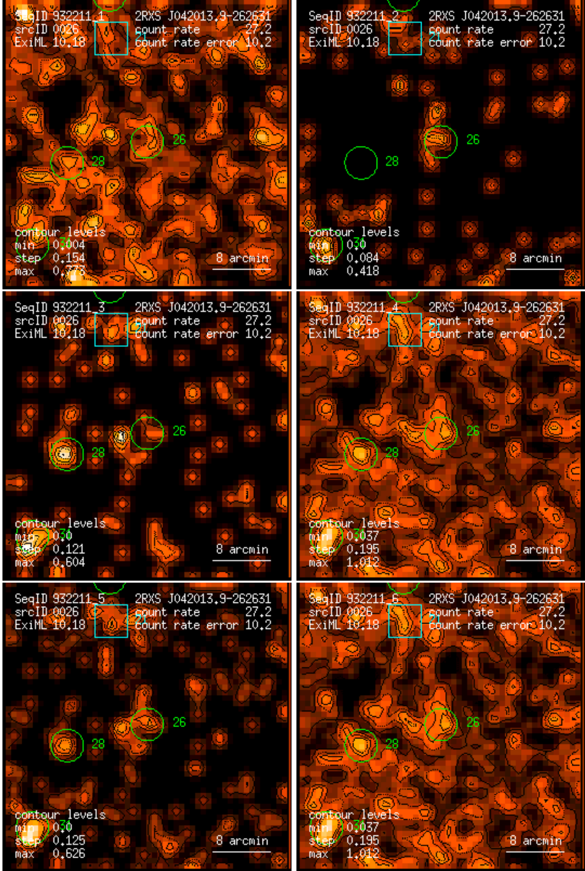
Figure 26: RASS 932211: detection 0026: band rate images, Gaussian filter: (1) PSPC channels 11 – 41, (2) 52 – 90, (3) 91 – 201, (4) 11 – 235, (5) 52 – 201, (6) 11 – 201. Broad band rates in counts/ks. Band rate contour levels in counts/ks/arcmin 2 .
