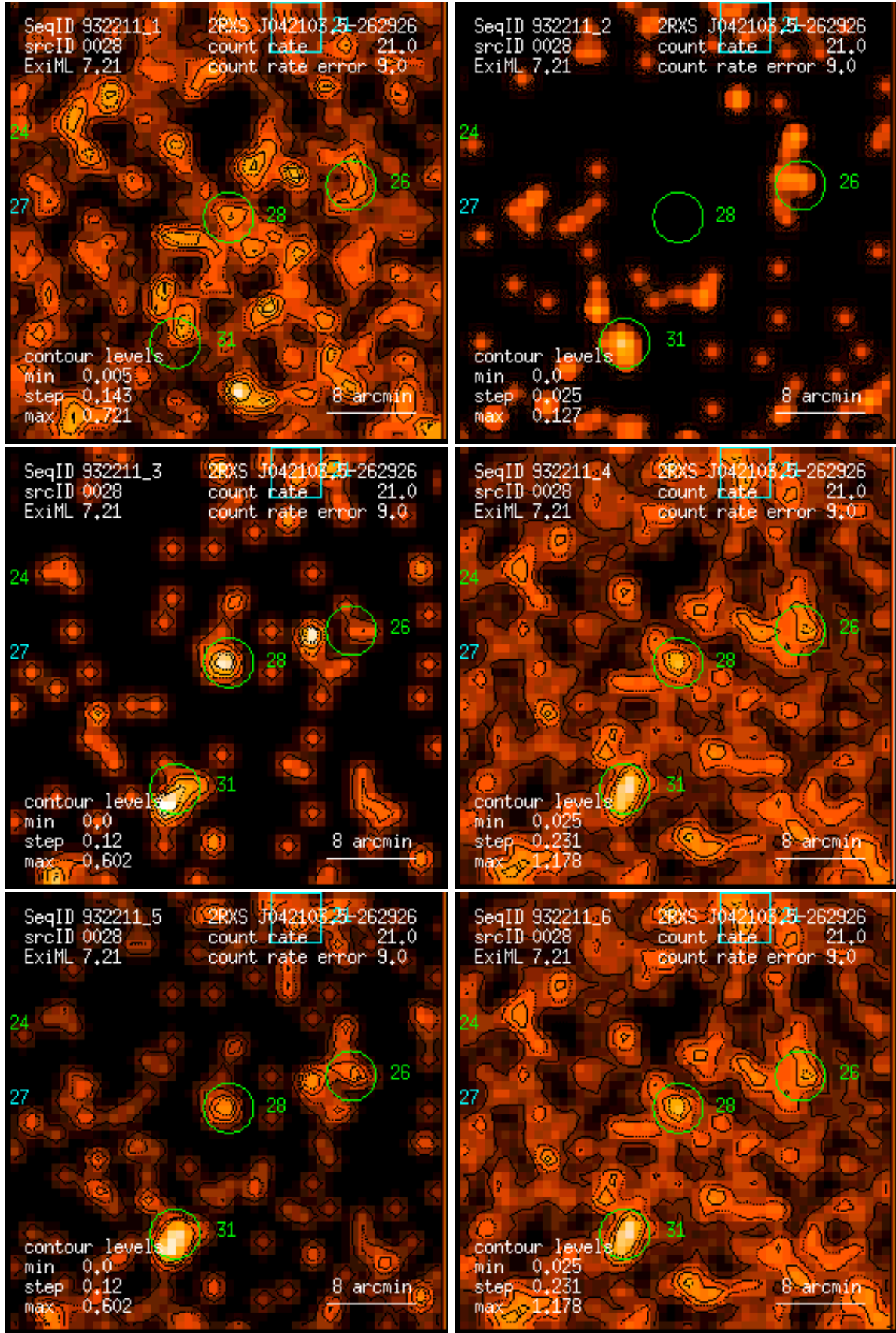
Figure 28: RASS 932211: detection 0028: band rate images, Gaussian filter: (1) PSPC channels 11 – 41, (2) 52 – 90, (3) 91 – 201, (4) 11 – 235, (5) 52 – 201, (6) 11 – 201. Broad band rates in counts/ks. Band rate contour levels in counts/ks/arcmin 2 .
