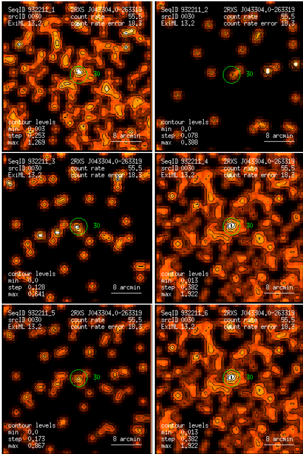
Figure 30: RASS 932211: detection 0030: band rate images, Gaussian filter: (1) PSPC channels 11 – 41, (2) 52 – 90, (3) 91 – 201, (4) 11 – 235, (5) 52 – 201, (6) 11 – 201. Broad band rates in counts/ks. Band rate contour levels in counts/ks/arcmin 2 .
