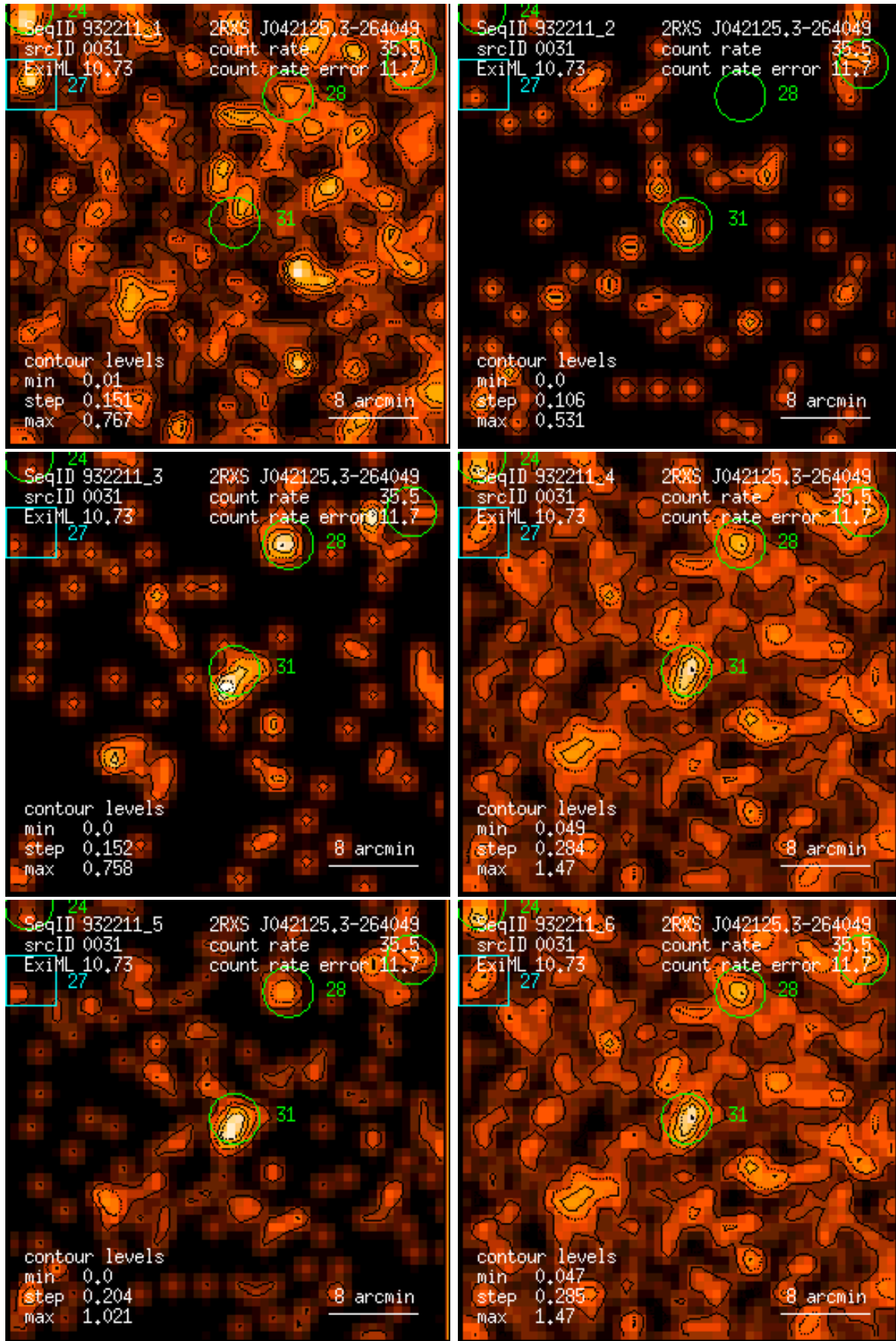
Figure 31: RASS 932211: detection 0031: band rate images, Gaussian filter: (1) PSPC channels 11 – 41, (2) 52 – 90, (3) 91 – 201, (4) 11 – 235, (5) 52 – 201, (6) 11 – 201. Broad band rates in counts/ks. Band rate contour levels in counts/ks/arcmin 2 .
