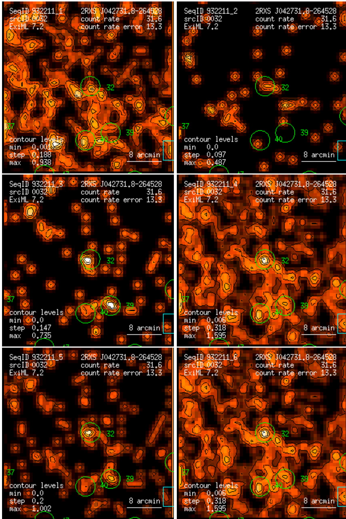
Figure 32: RASS 932211: detection 0032: band rate images, Gaussian filter: (1) PSPC channels 11 – 41, (2) 52 – 90, (3) 91 – 201, (4) 11 – 235, (5) 52 – 201, (6) 11 – 201. Broad band rates in counts/ks. Band rate contour levels in counts/ks/arcmin 2 .
