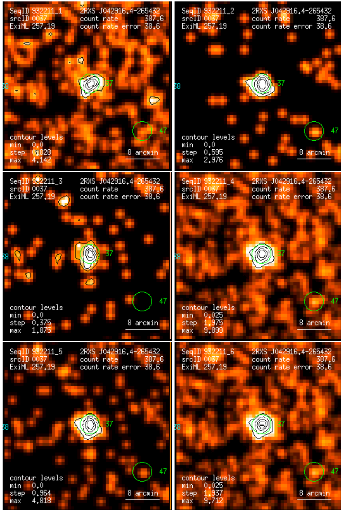
Figure 37: RASS 932211: detection 0037: band rate images, Gaussian filter: (1) PSPC channels 11 – 41, (2) 52 – 90, (3) 91 – 201, (4) 11 – 235, (5) 52 – 201, (6) 11 – 201. Broad band rates in counts/ks. Band rate contour levels in counts/ks/arcmin 2 .
