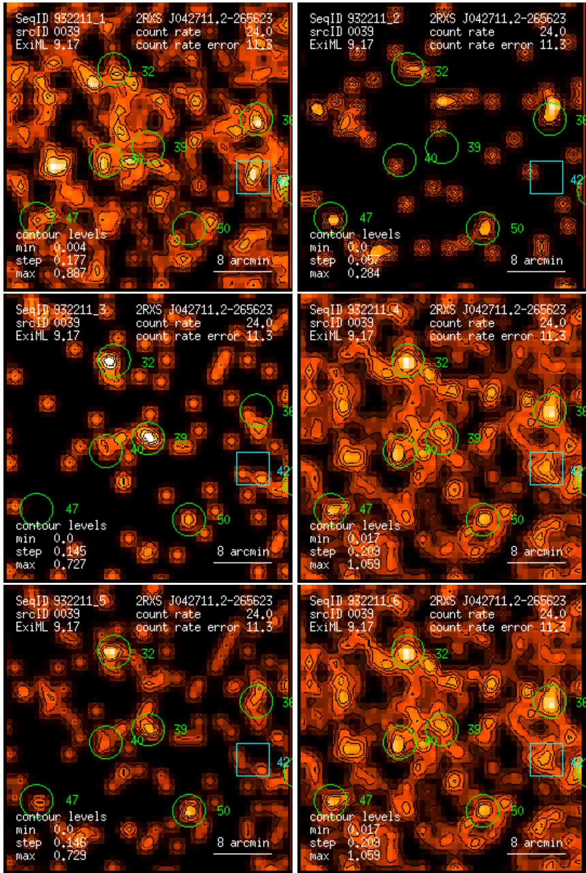
Figure 39: RASS 932211: detection 0039: band rate images, Gaussian filter: (1) PSPC channels 11 – 41, (2) 52 – 90, (3) 91 – 201, (4) 11 – 235, (5) 52 – 201, (6) 11 – 201. Broad band rates in counts/ks. Band rate contour levels in counts/ks/arcmin 2 .
