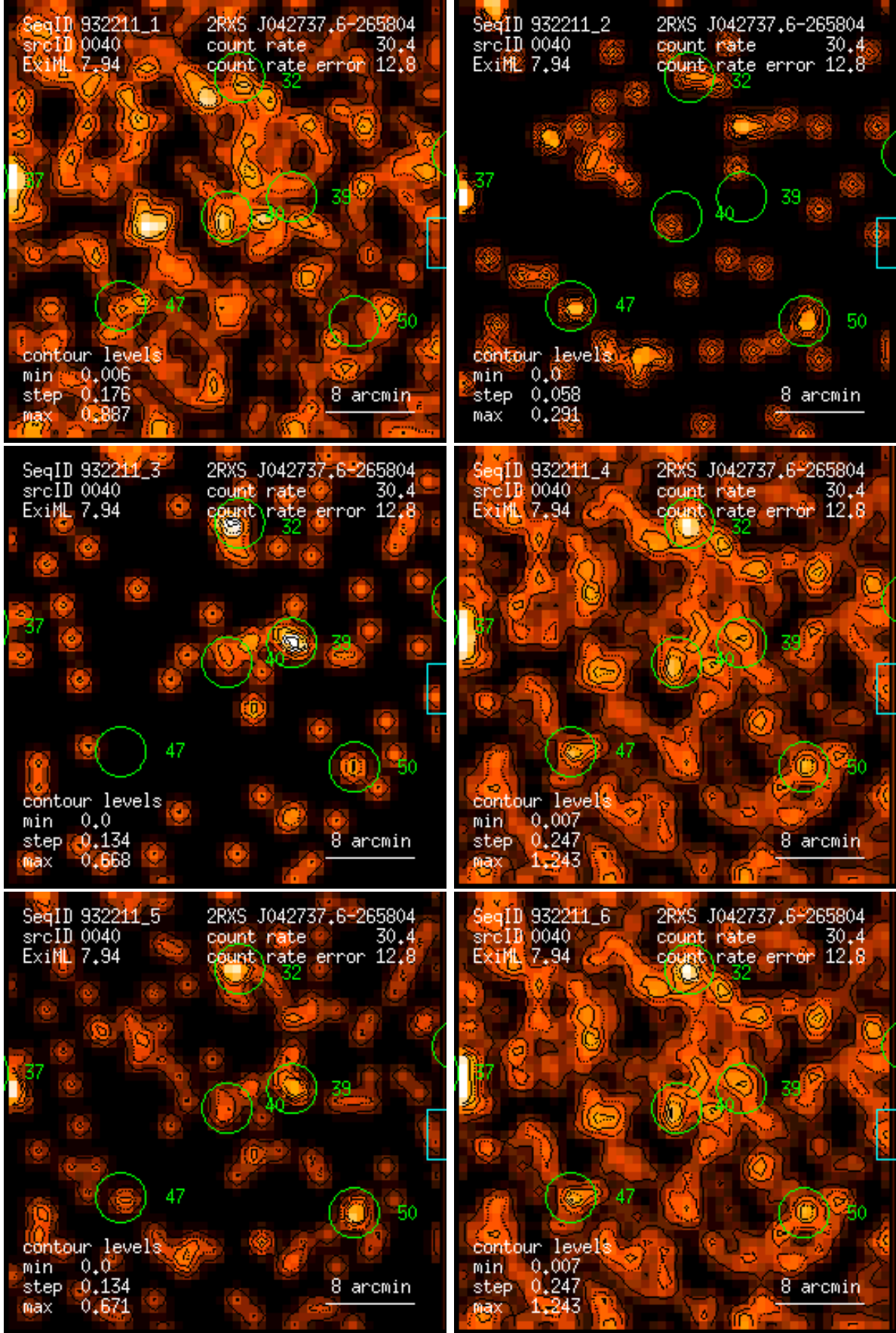
Figure 40: RASS 932211: detection 0040: band rate images, Gaussian filter: (1) PSPC channels 11 – 41, (2) 52 – 90, (3) 91 – 201, (4) 11 – 235, (5) 52 – 201, (6) 11 – 201. Broad band rates in counts/ks. Band rate contour levels in counts/ks/arcmin 2 .
