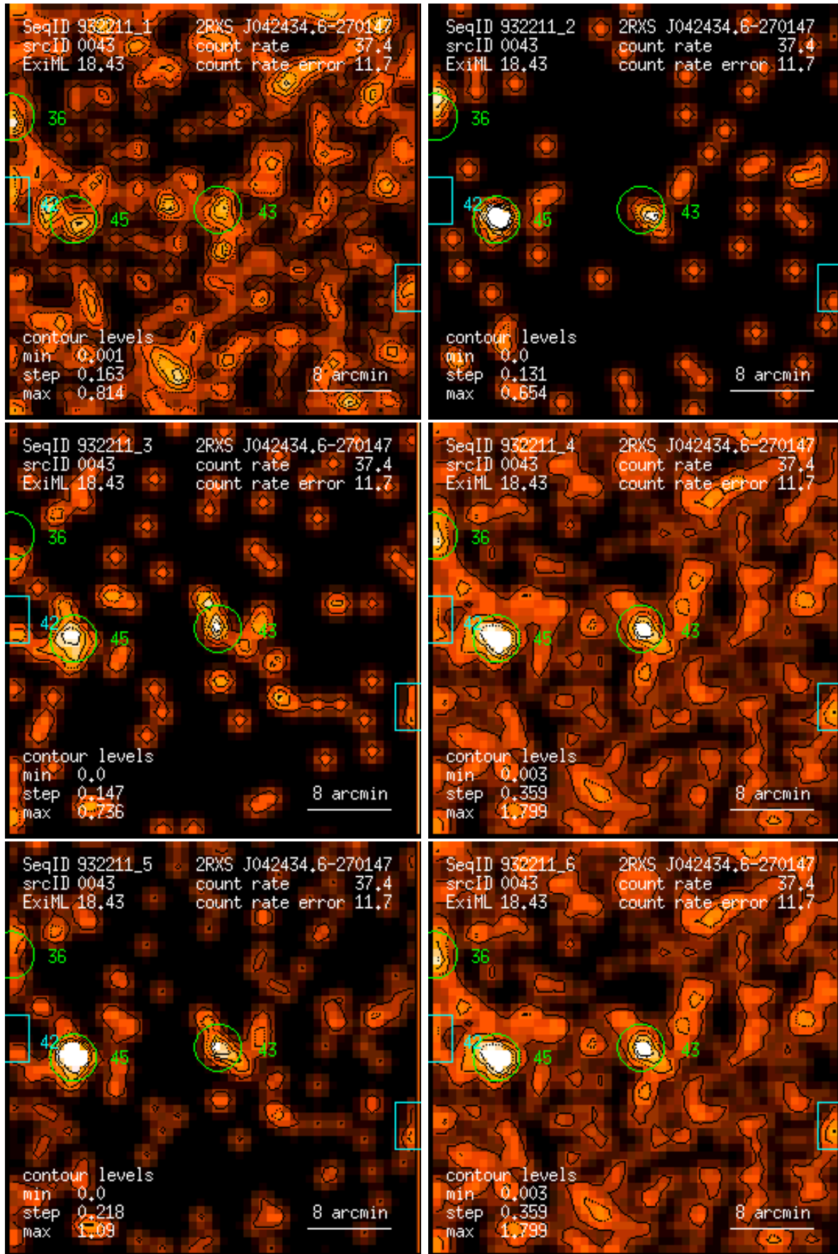
Figure 43: RASS 932211: detection 0043: band rate images, Gaussian filter: (1) PSPC channels 11 – 41, (2) 52 – 90, (3) 91 – 201, (4) 11 – 235, (5) 52 – 201, (6) 11 – 201. Broad band rates in counts/ks. Band rate contour levels in counts/ks/arcmin 2 .
