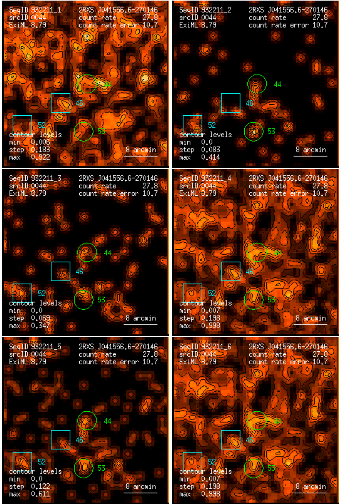
Figure 44: RASS 932211: detection 0044: band rate images, Gaussian filter: (1) PSPC channels 11 – 41, (2) 52 – 90, (3) 91 – 201, (4) 11 – 235, (5) 52 – 201, (6) 11 – 201. Broad band rates in counts/ks. Band rate contour levels in counts/ks/arcmin 2 .
