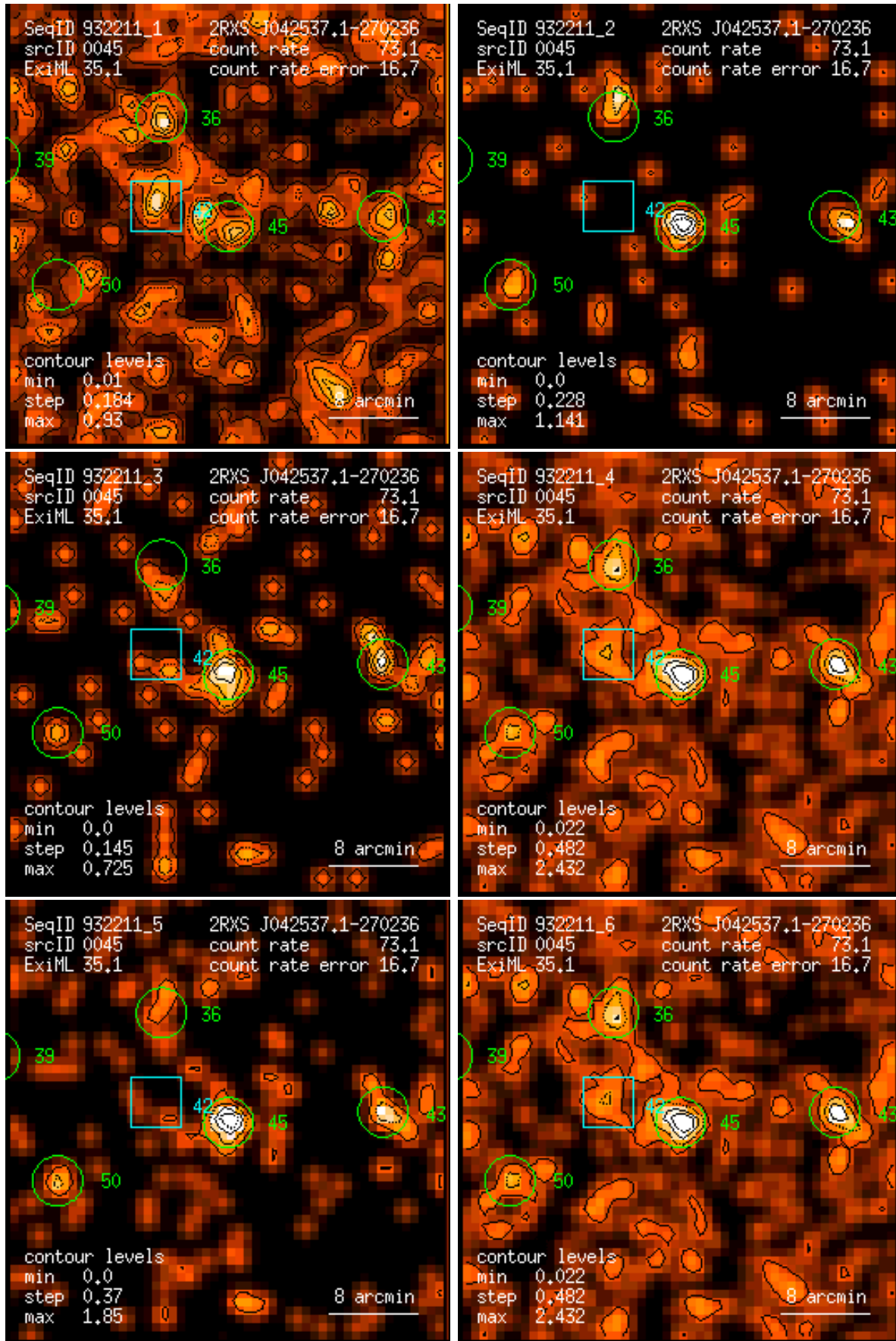
Figure 45: RASS 932211: detection 0045: band rate images, Gaussian filter: (1) PSPC channels 11 – 41, (2) 52 – 90, (3) 91 – 201, (4) 11 – 235, (5) 52 – 201, (6) 11 – 201. Broad band rates in counts/ks. Band rate contour levels in counts/ks/arcmin 2 .
