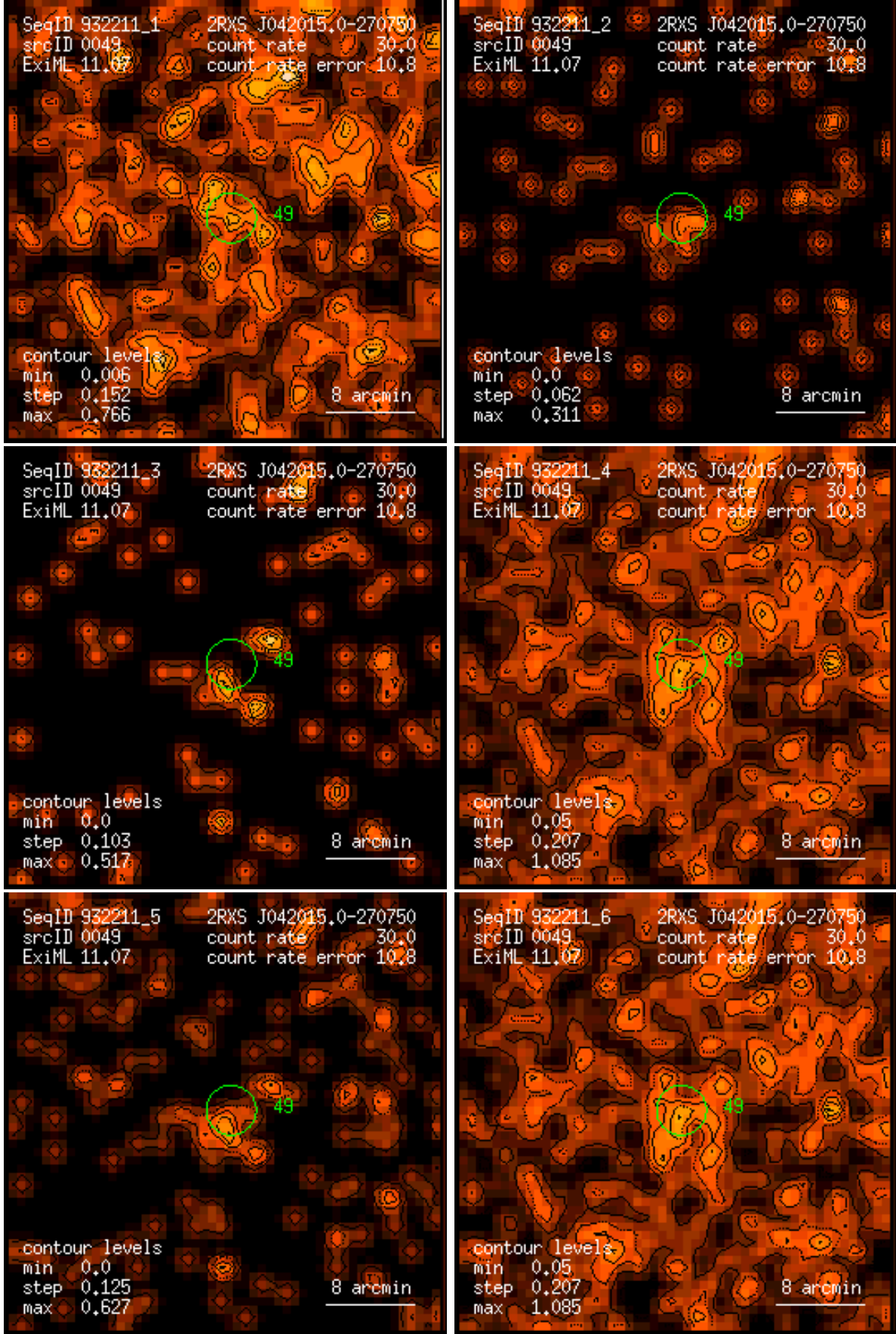
Figure 49: RASS 932211: detection 0049: band rate images, Gaussian filter: (1) PSPC channels 11 – 41, (2) 52 – 90, (3) 91 – 201, (4) 11 – 235, (5) 52 – 201, (6) 11 – 201. Broad band rates in counts/ks. Band rate contour levels in counts/ks/arcmin 2 .
