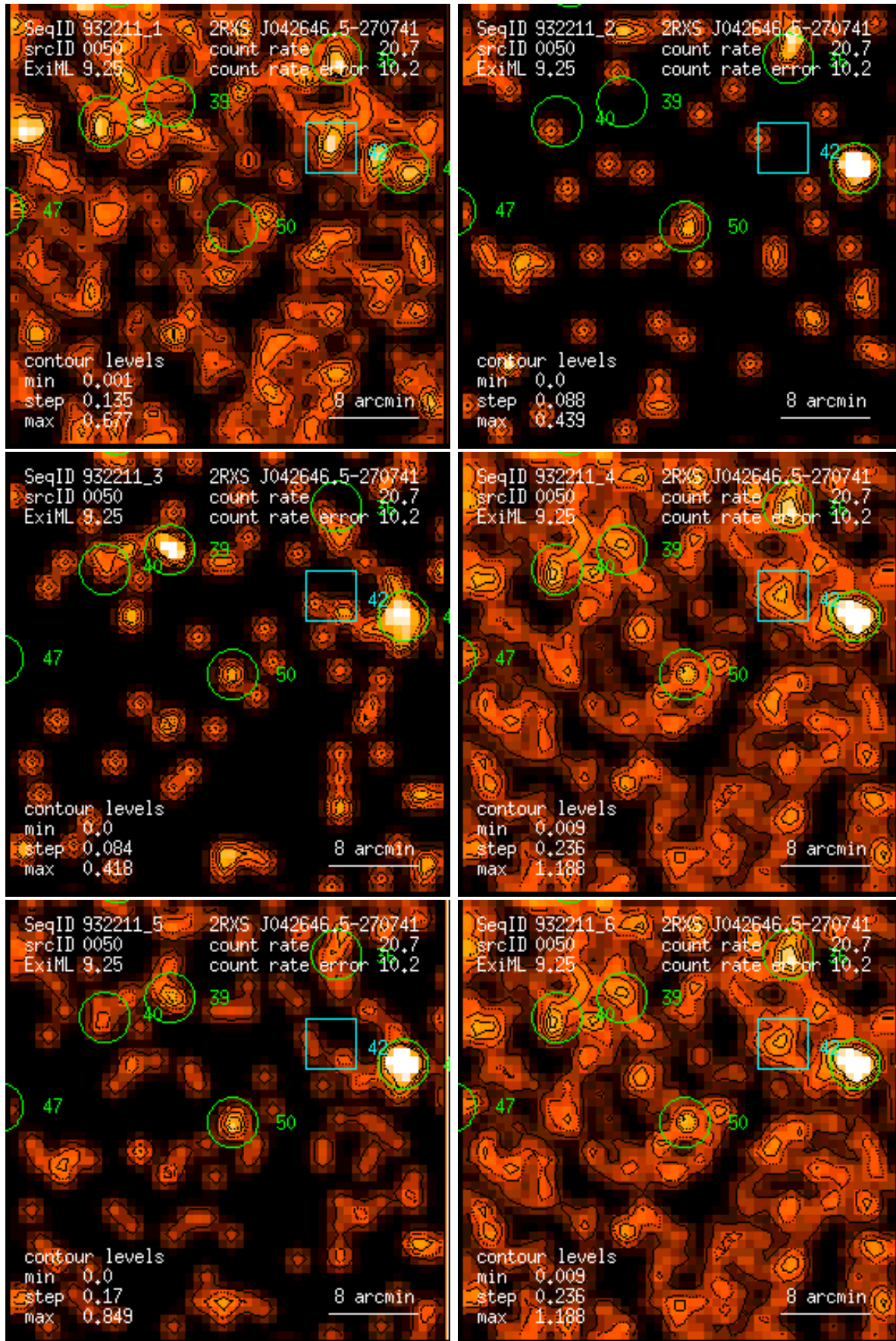
Figure 50: RASS 932211: detection 0050: band rate images, Gaussian filter: (1) PSPC channels 11 – 41, (2) 52 – 90, (3) 91 – 201, (4) 11 – 235, (5) 52 – 201, (6) 11 – 201. Broad band rates in counts/ks. Band rate contour levels in counts/ks/arcmin 2 .
