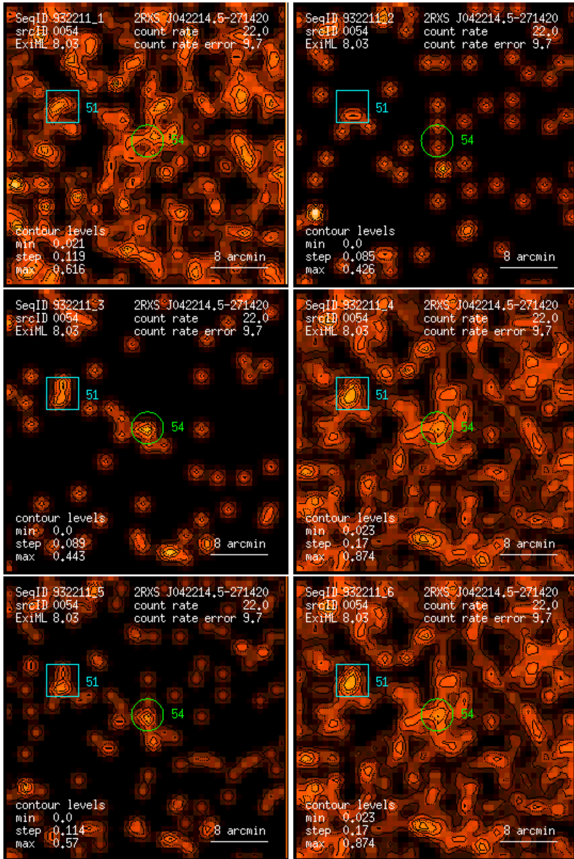
Figure 54: RASS 932211: detection 0054: band rate images, Gaussian filter: (1) PSPC channels 11 – 41, (2) 52 – 90, (3) 91 – 201, (4) 11 – 235, (5) 52 – 201, (6) 11 – 201. Broad band rates in counts/ks. Band rate contour levels in counts/ks/arcmin 2 .
