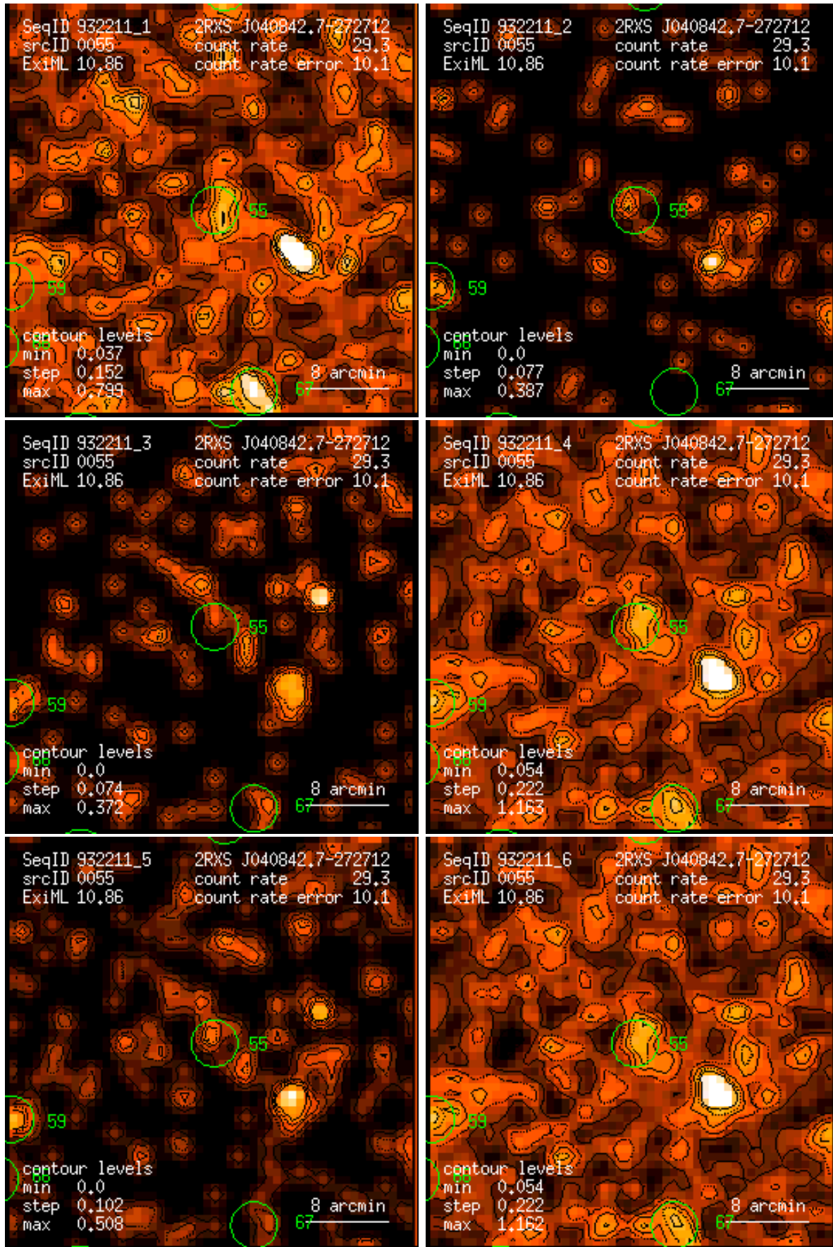
Figure 55: RASS 932211: detection 0055: band rate images, Gaussian filter: (1) PSPC channels 11 – 41, (2) 52 – 90, (3) 91 – 201, (4) 11 – 235, (5) 52 – 201, (6) 11 – 201. Broad band rates in counts/ks. Band rate contour levels in counts/ks/arcmin 2 .
