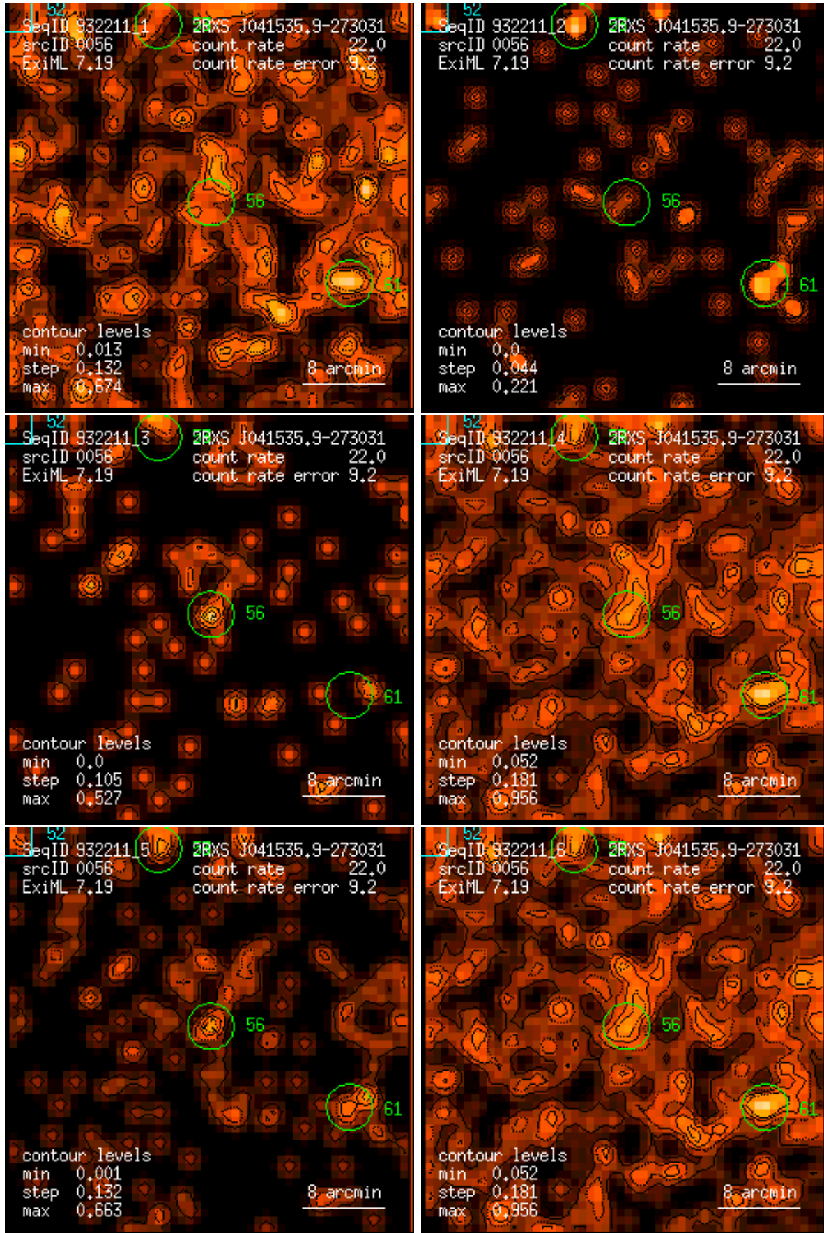
Figure 56: RASS 932211: detection 0056: band rate images, Gaussian filter: (1) PSPC channels 11 – 41, (2) 52 – 90, (3) 91 – 201, (4) 11 – 235, (5) 52 – 201, (6) 11 – 201. Broad band rates in counts/ks. Band rate contour levels in counts/ks/arcmin 2 .
