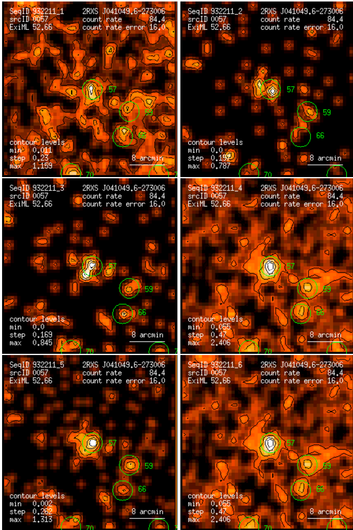
Figure 57: RASS 932211: detection 0057: band rate images, Gaussian filter: (1) PSPC channels 11 – 41, (2) 52 – 90, (3) 91 – 201, (4) 11 – 235, (5) 52 – 201, (6) 11 – 201. Broad band rates in counts/ks. Band rate contour levels in counts/ks/arcmin 2 .
