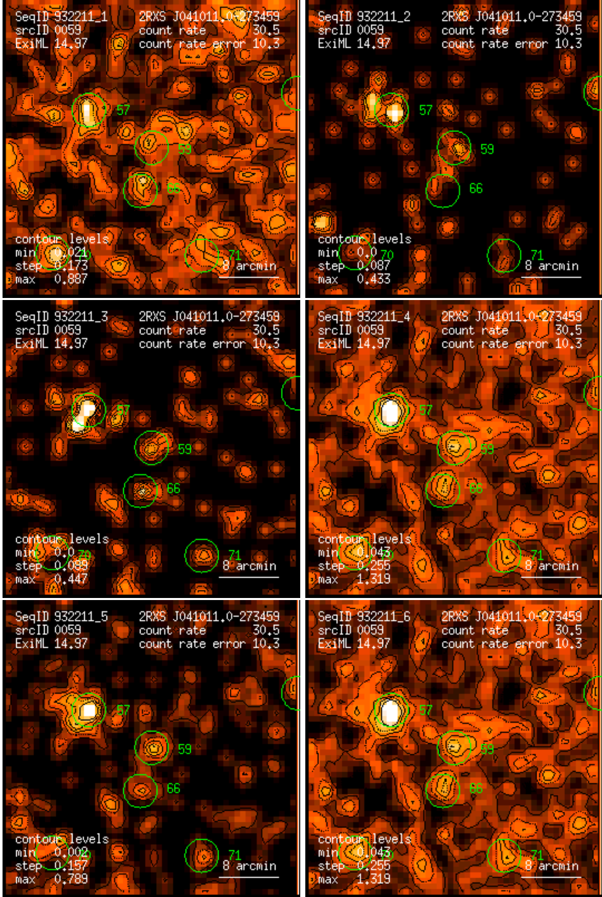
Figure 59: RASS 932211: detection 0059: band rate images, Gaussian filter: (1) PSPC channels 11 – 41, (2) 52 – 90, (3) 91 – 201, (4) 11 – 235, (5) 52 – 201, (6) 11 – 201. Broad band rates in counts/ks. Band rate contour levels in counts/ks/arcmin 2 .
